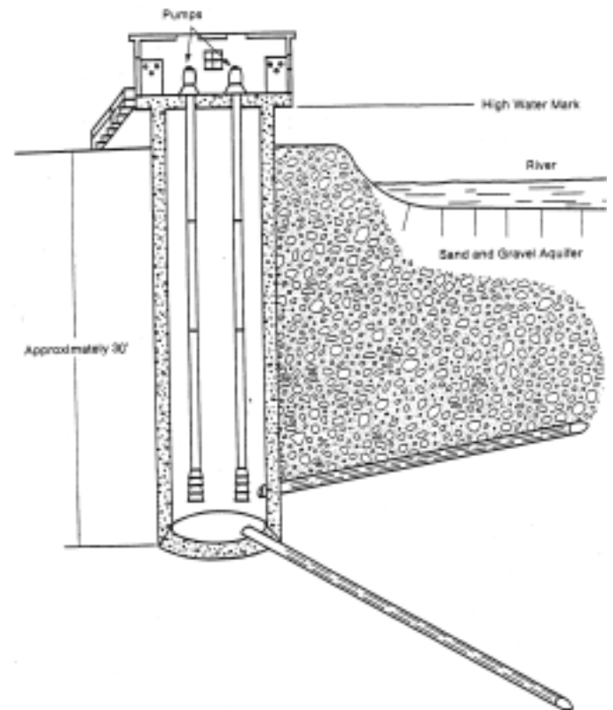
FIGURE 2—Collector well schematic diagram.
