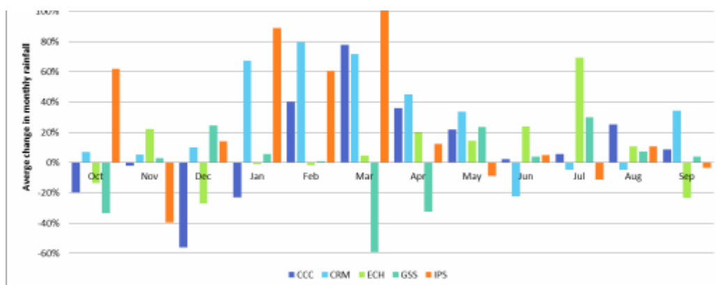
Figure 4 Predicted rainfall changes in the Berg River catchment, South Africa, under five GCMs
