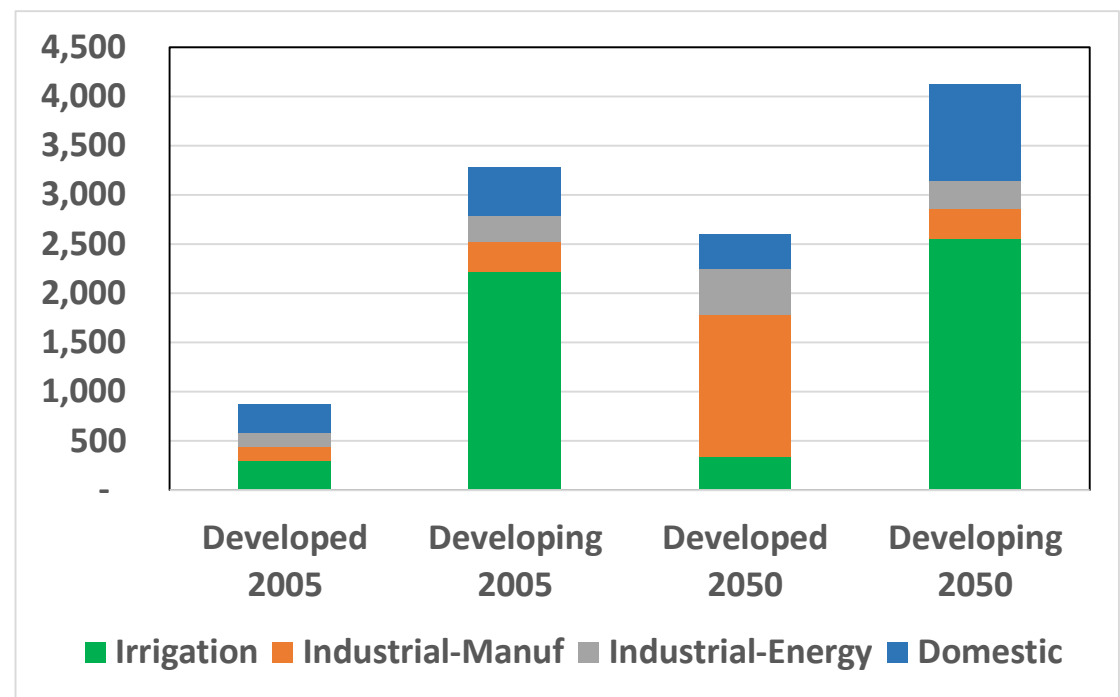
Figure 5 Global water demand: 2005 and 2050
