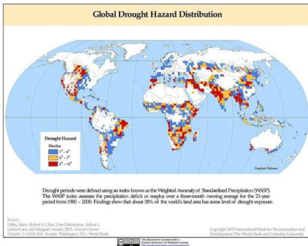
Figure 2 Global Drought Hazard Distribution
