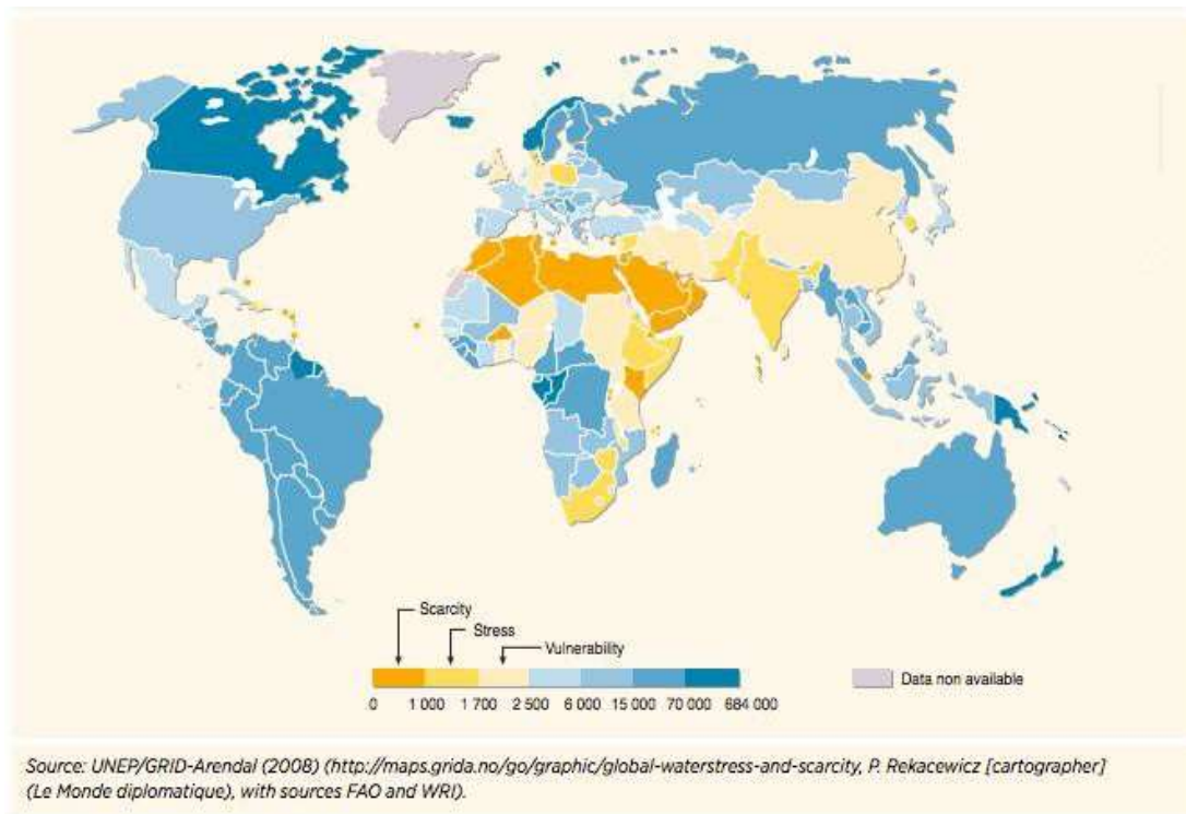
Figure 8 Freshwater availability ( \text{m}^3 per person per year, 2007)
