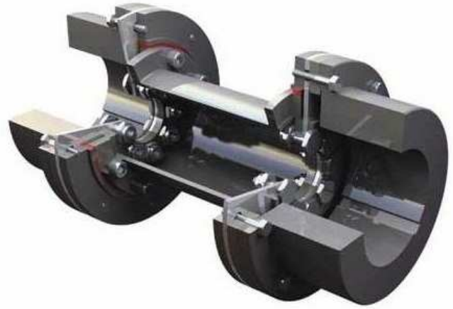
Figure 3.2: Typical Flexible Membrane Coupling
