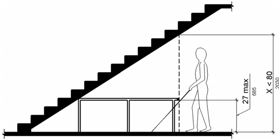
Figure 307.4 Vertical Clearance
