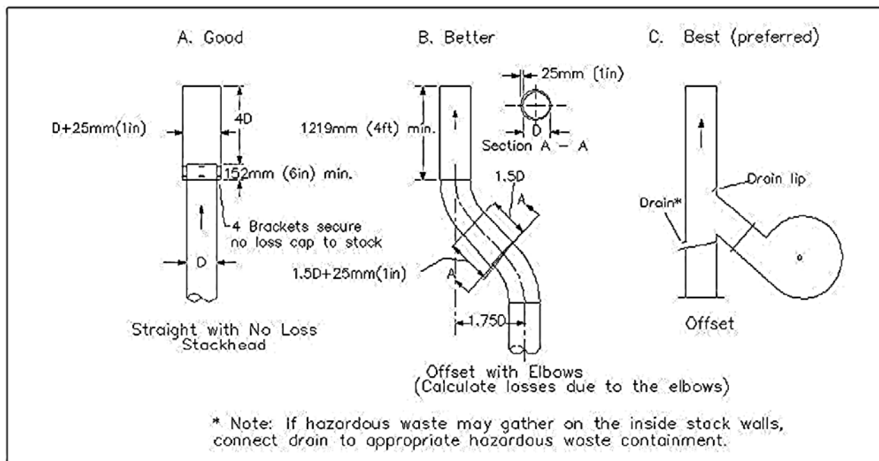
Exhaust Stack Designs
