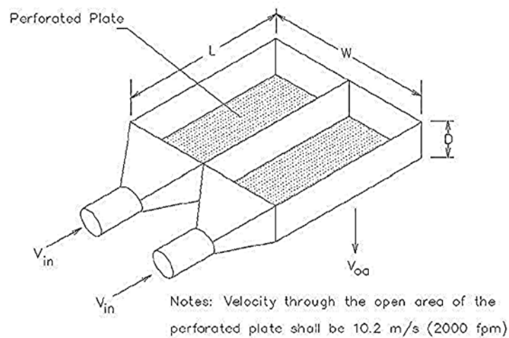
Plenum Design without Perforated Duct
