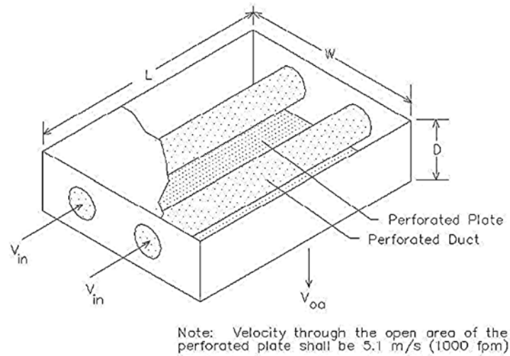
Plenum Design with Perforated Duct
