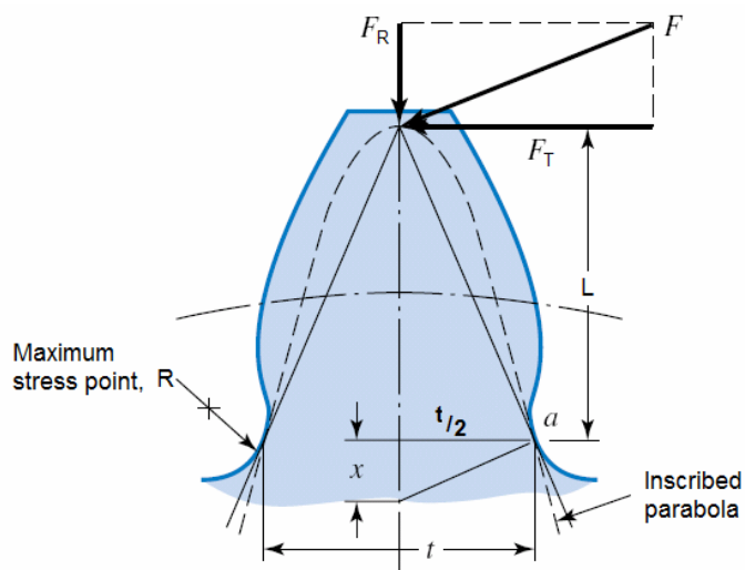
Gear Tooth as Cantilever
