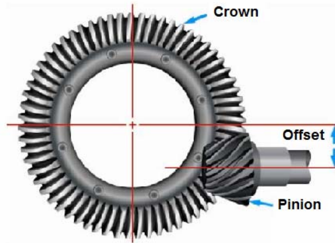
Hypoid Gears
