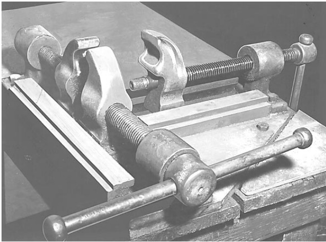
Figure 5-6.—A rigger's vise.
