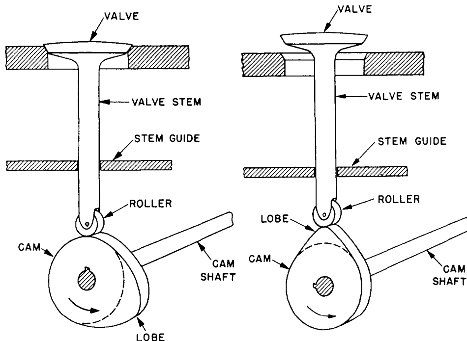
Figure 6-12.-Camdriven valve.
