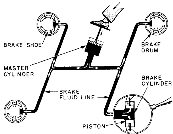
Figure 10-6.-Hydraulic brakes.
