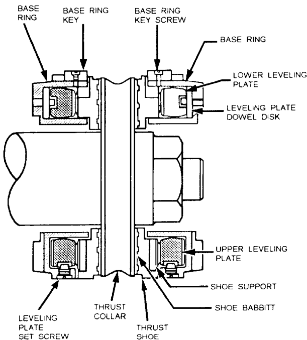
Figure 11-2.-Kingsbury pivoted-shoe thrust bearing.
