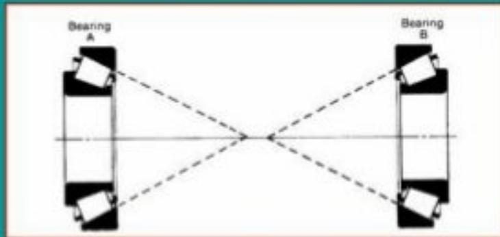
Indirect mounting
