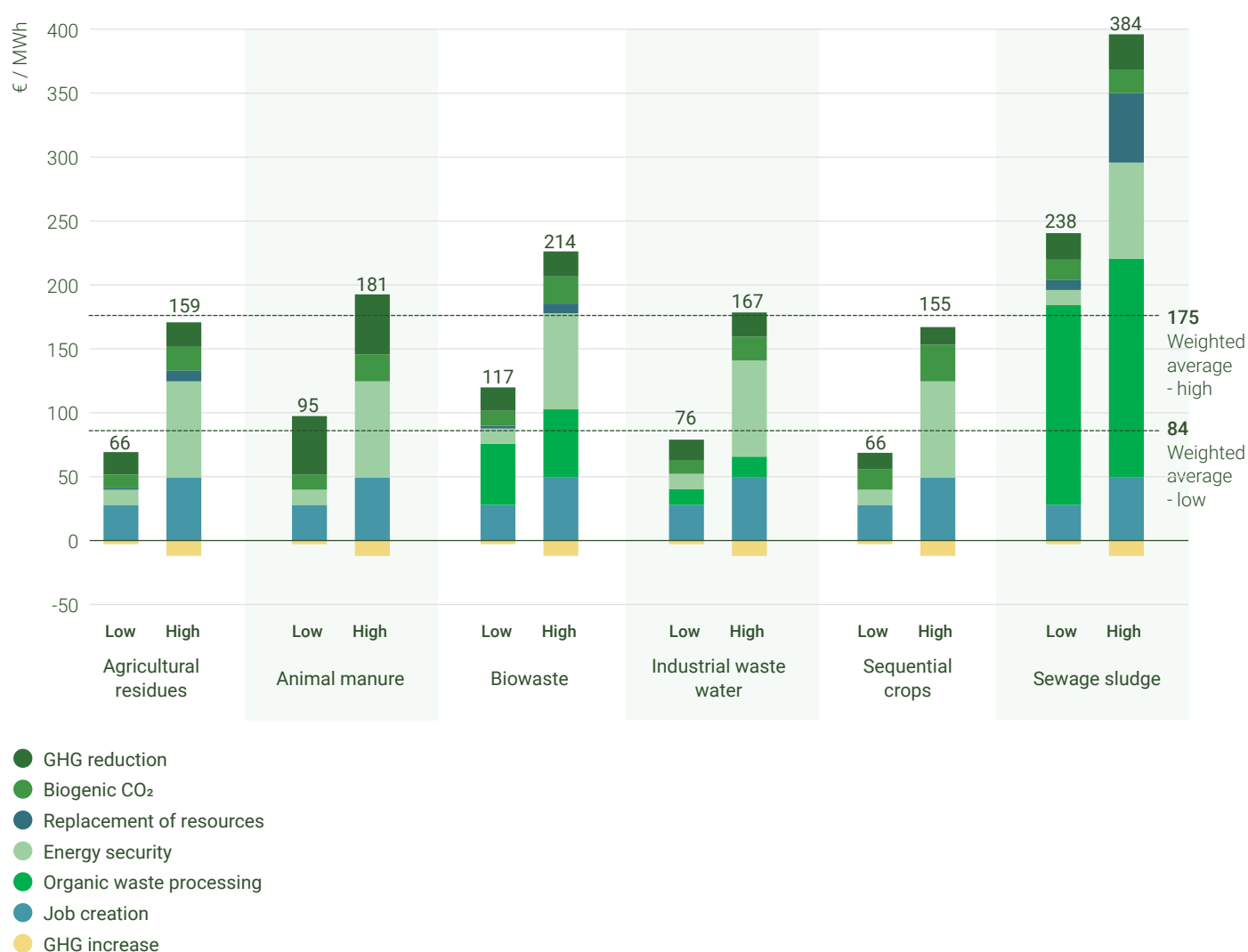
Figure 6.17 | Anaerobic digestion: Externality benefit per feedstock for each externality (€/MWh)
