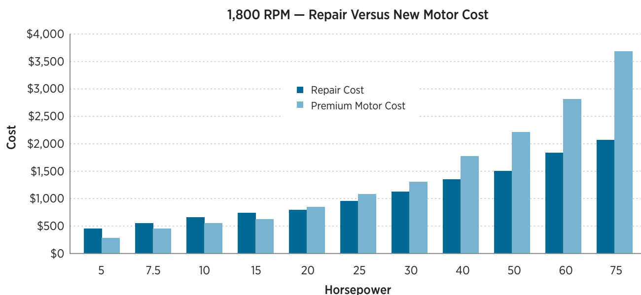
Figure 7-1. Repair and New Premium Efficiency Motor Costs (for 1,800 RPM TEFC Motors, 2011 Prices)
