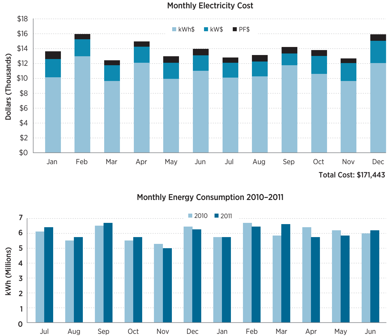
Figure 2-1. Energy Use Profile Reports. Illustration from EM4MDS
