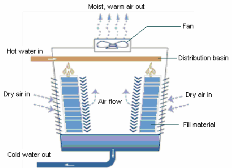
Crossflow Type Design
