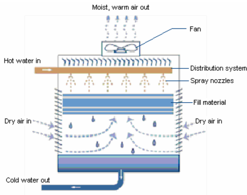
Counterflow Type Design
