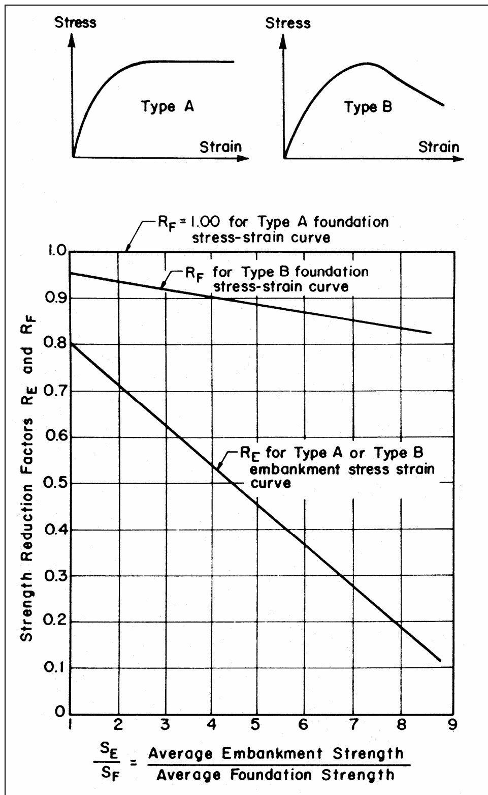
Figure 7-5. Peak strength correction factors for both embankment and foundation to prevent progressive failure in the foundation for embankments on soft clay foundations (Duncan and Buchignani 1975)
