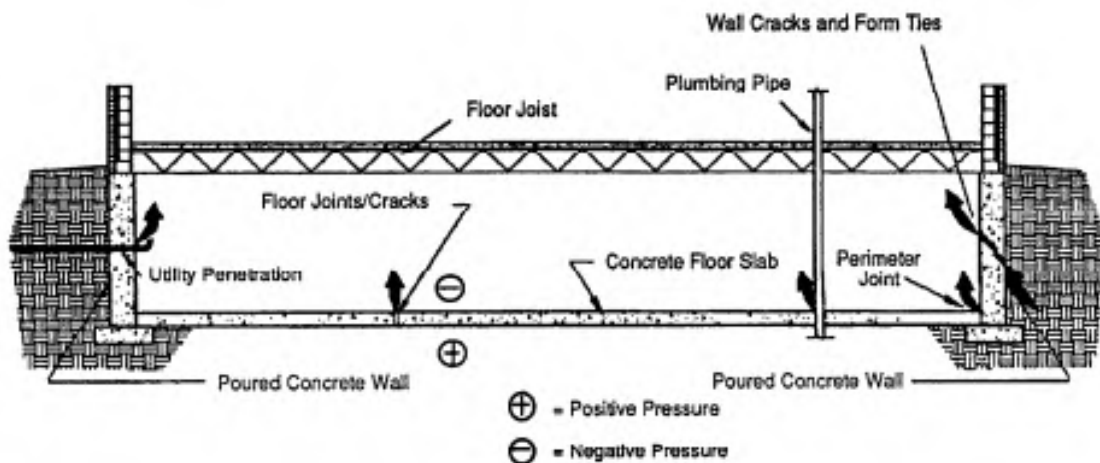
Figure 1-3. Typical radon entry routes in slab-on-grade construction.
