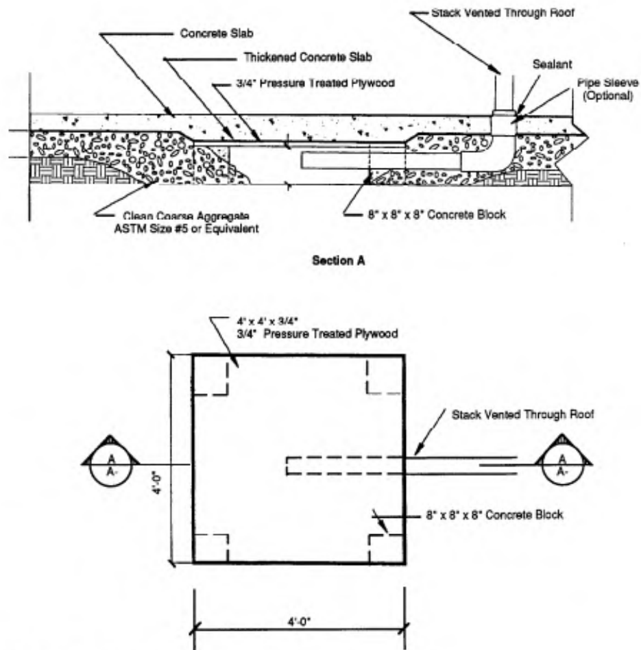
Figure 2-5. Radon suction pit. Not to scale.
