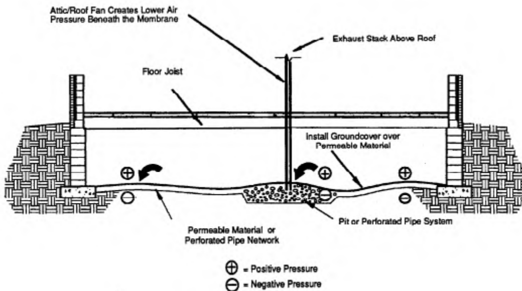
Figure 2-7. Submembrane depressurization in crawl space.
