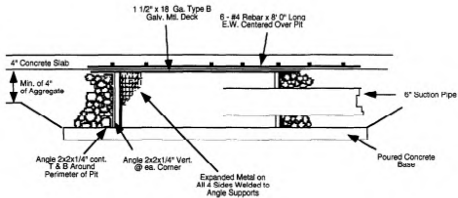
Figure 2-12. Revised subslab suction pit.
