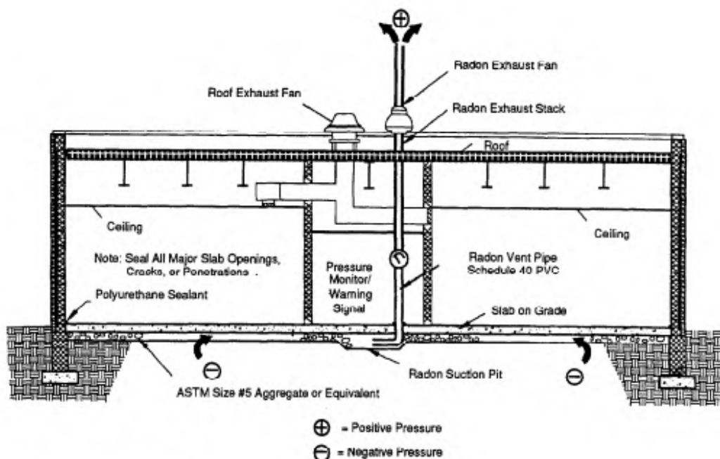
Figure 2-1. Typical subslab depressurization system. Not to scale.
