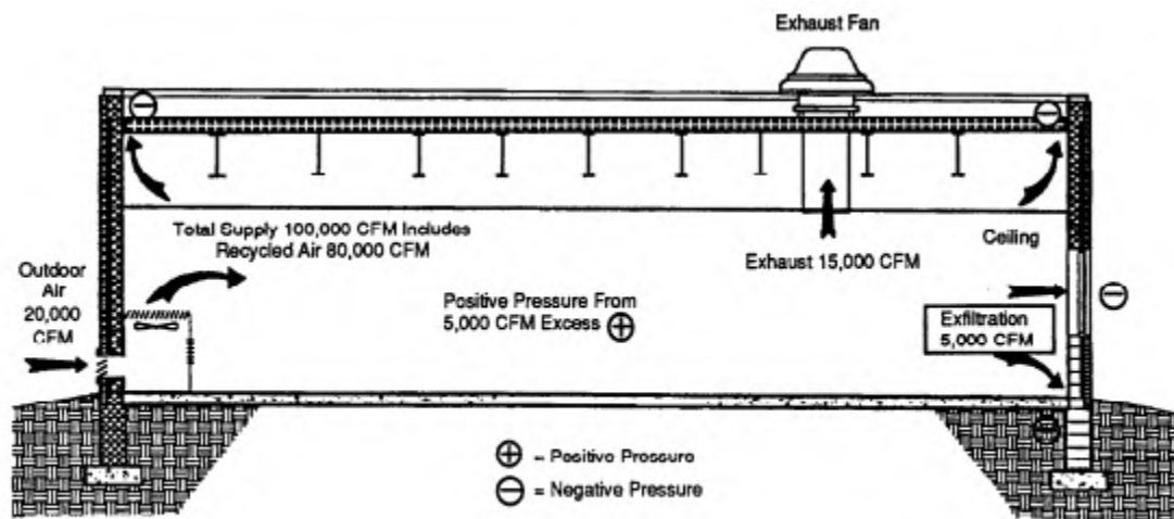
Figure 2-8. Building positive pressurization with HVAC system.
