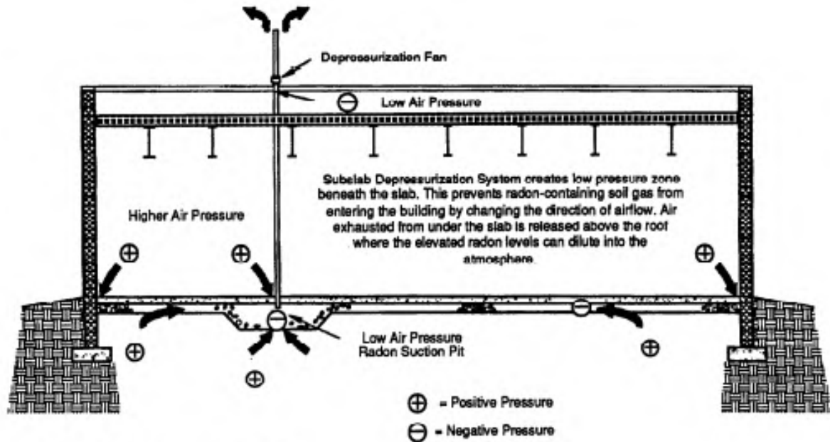
Figure 1-6. Subslab depressurization theory.
