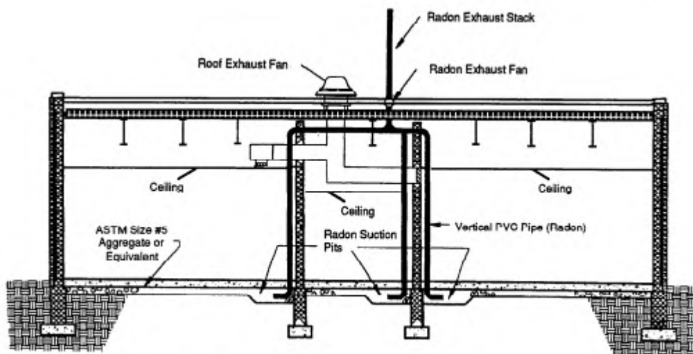
Figure 2-4b. Section 1 (corresponds to Figures 2-3c and d). Not to scale.
