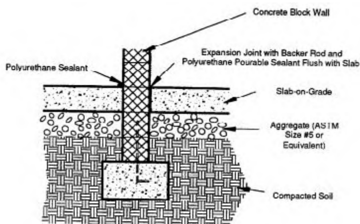
Figure 2-2a. Interior footing/foundation wall. Not to scale.
