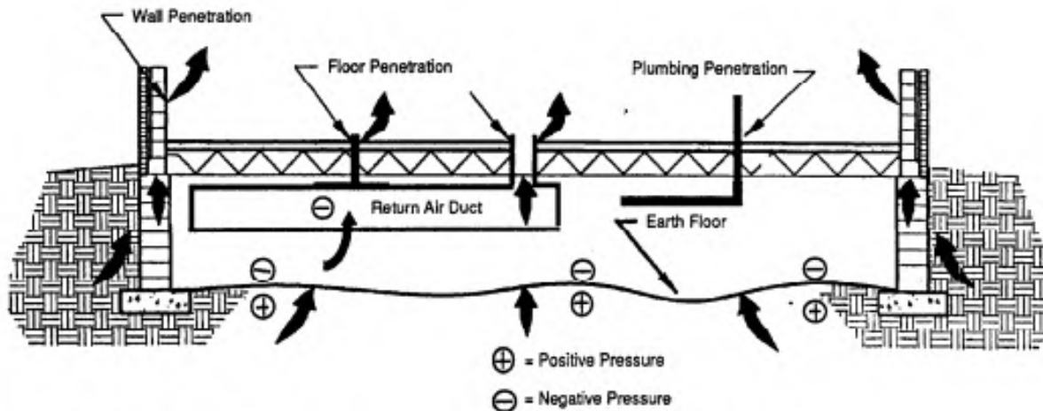
Figure 1-5. Typical crawl space foundation entry routes.
