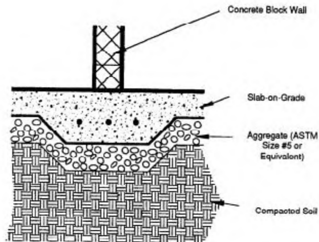
Figure 2-2b. Thickened slab footing. Not to scale.
