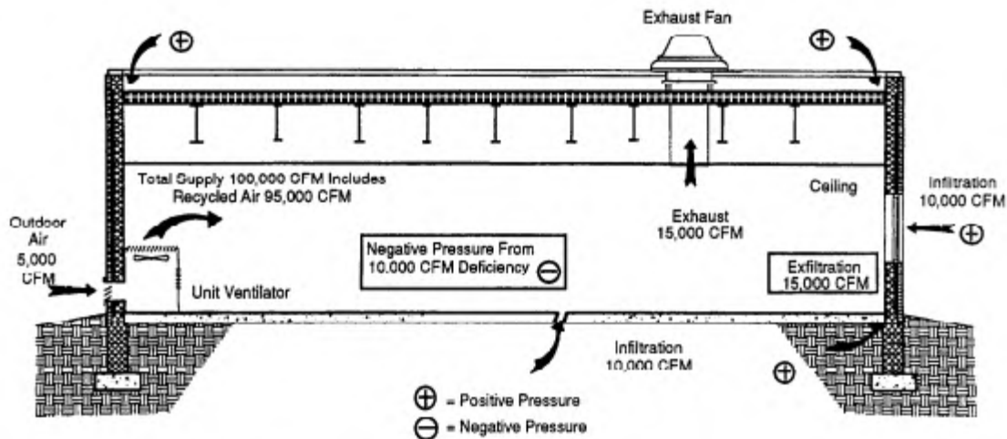
Figure 2-9. Example of building depressurization with HVAC system.
