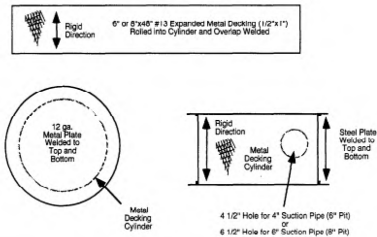
Figure 2-13. Smaller subslab suction pit.
