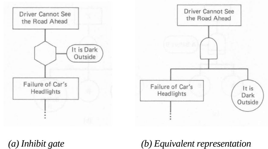
Figure 12: Inhibit gate
