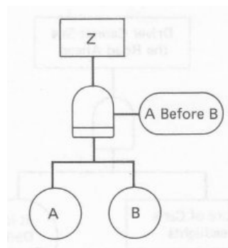
(a) Priority AND gate
