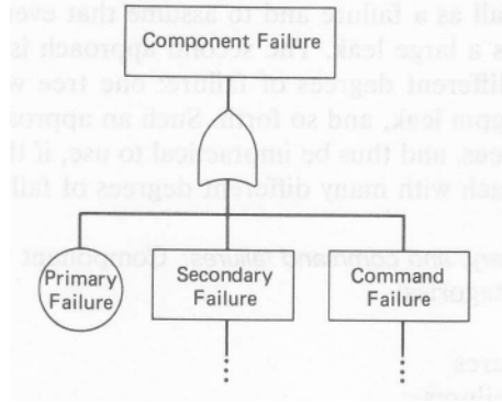
Figure 15: Resolution of a component failure into primary, secondary, and command failures
