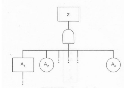
Figure 7: AND Gate
