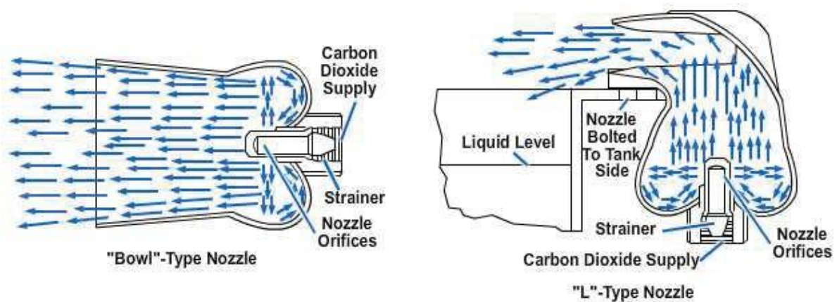
Figure 4-26 – Types of CO 2 nozzles.
