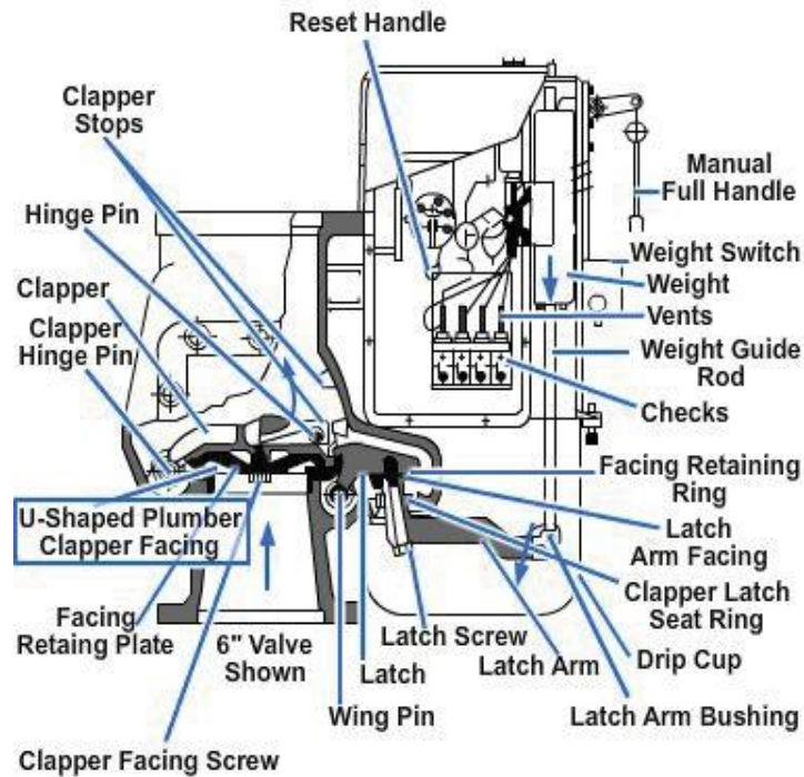
Figure 4-9 – Deluge valve.
