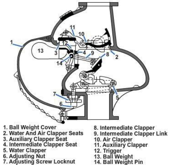
Figure 4-7 – Mechanical dry pipe valve.
