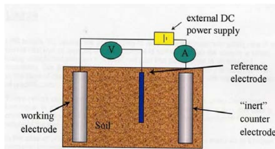
Figure 6-2. LPR Ferguson-Nicholas Cell
