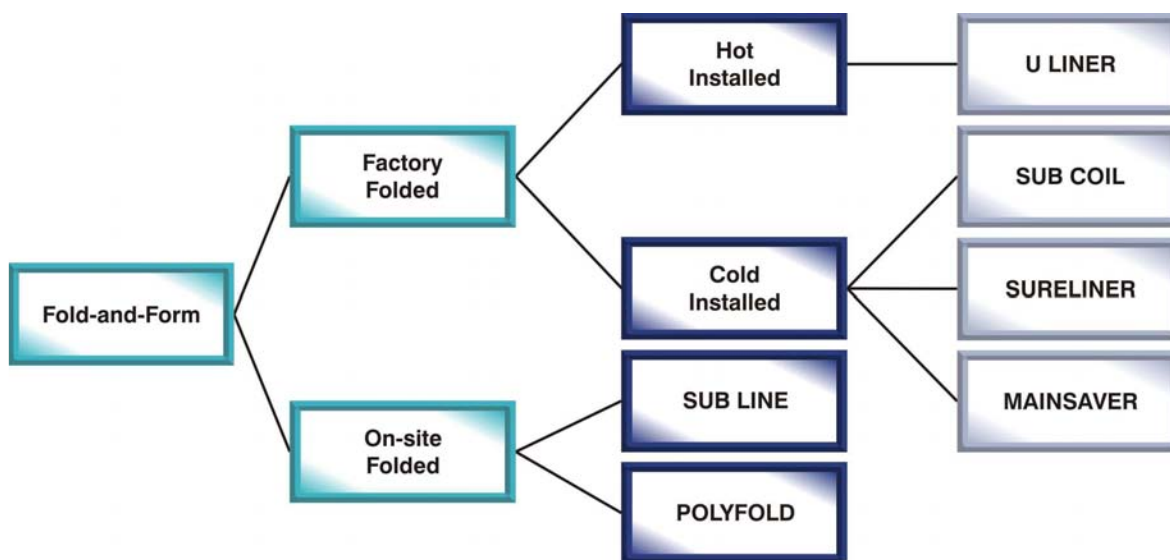
Figure 3-13. Summary of Fold-and-Form Close-Fit Lining Technologies
