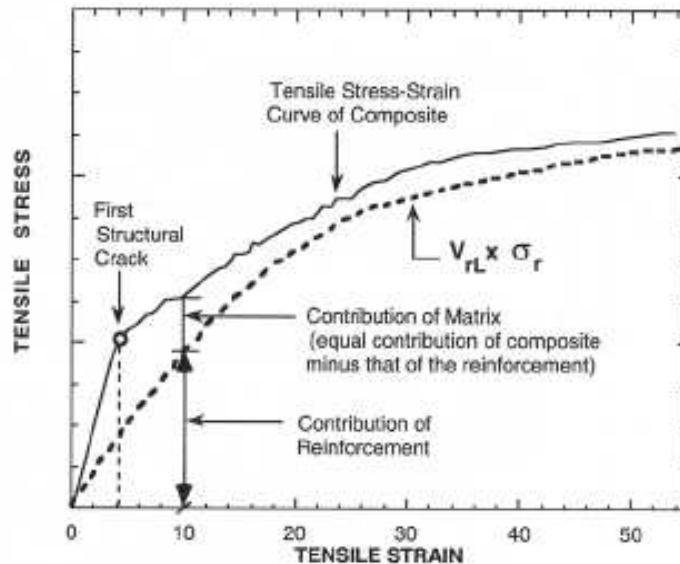
Figure 3-8. Typical Stress Strain Curve for Ferrocement (Newman, 2000)
