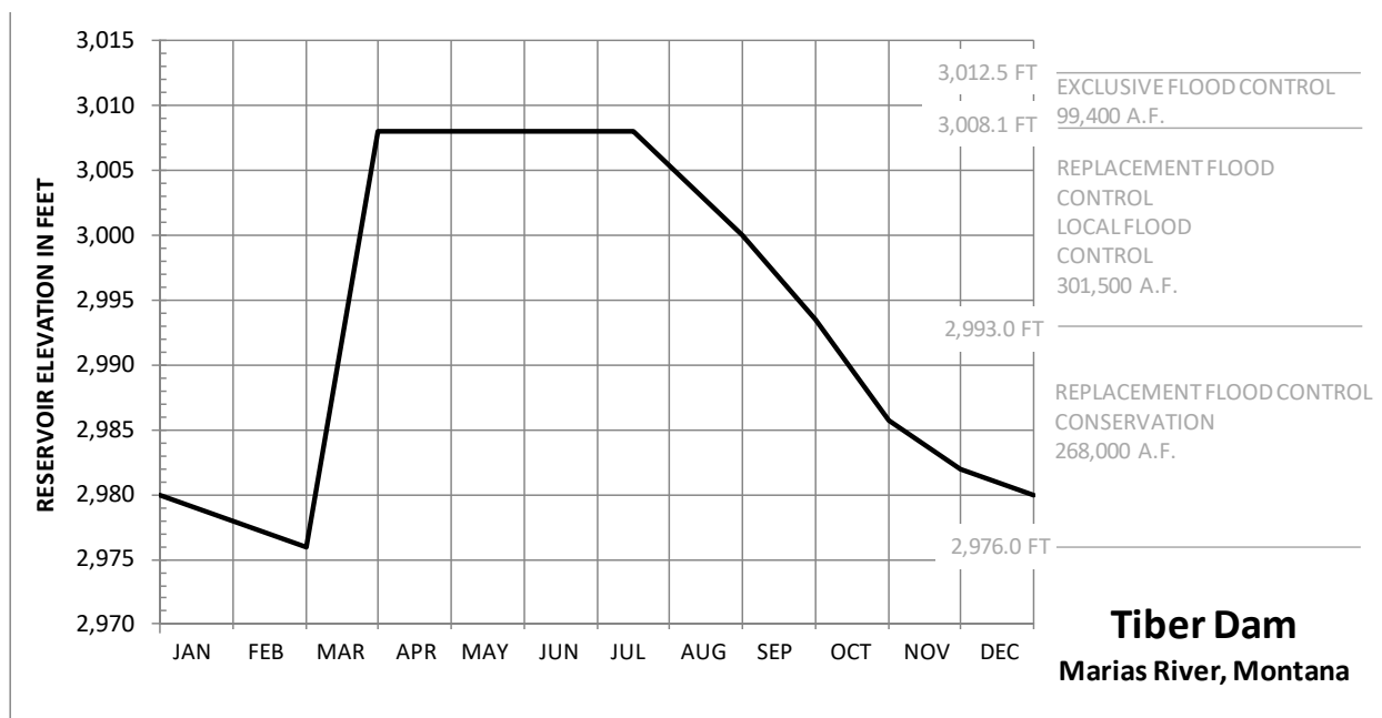
Figure 4-1. Guide Curve for Tiber Dam.
