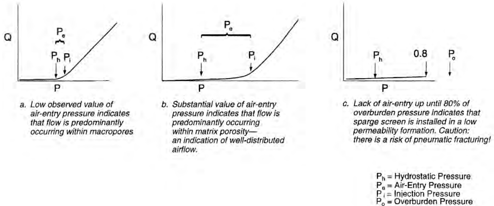
Figure 4-3. Interpretations of air-entry pressure from flow vs. pressure data.
