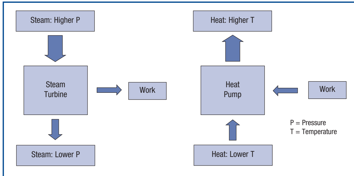
Figure 1.1: Comparison of Steam-Turbine and Heat-Pump Operating Principles
