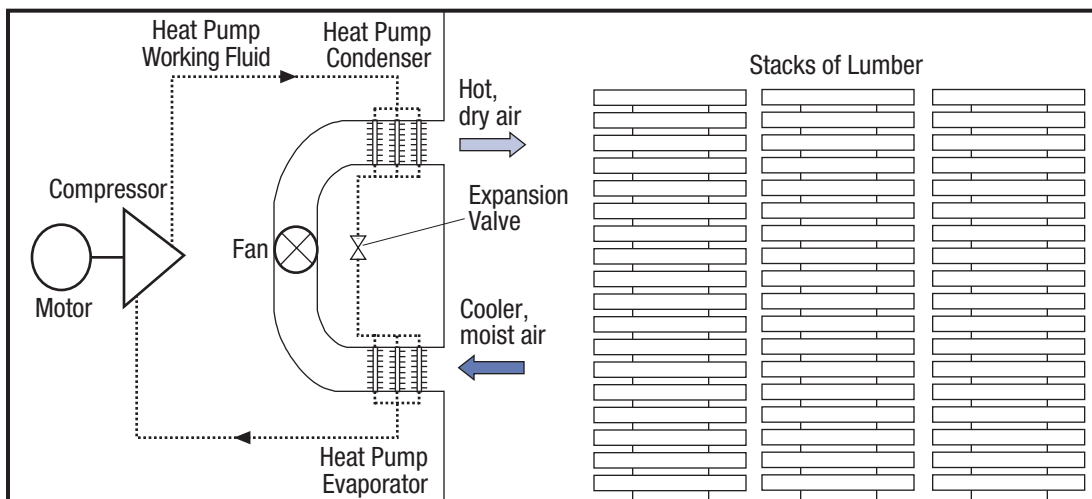
Figure 2.1b: Simplified Schematic of Closed-Cycle Heat-Pump Application for Lumber-Drying
