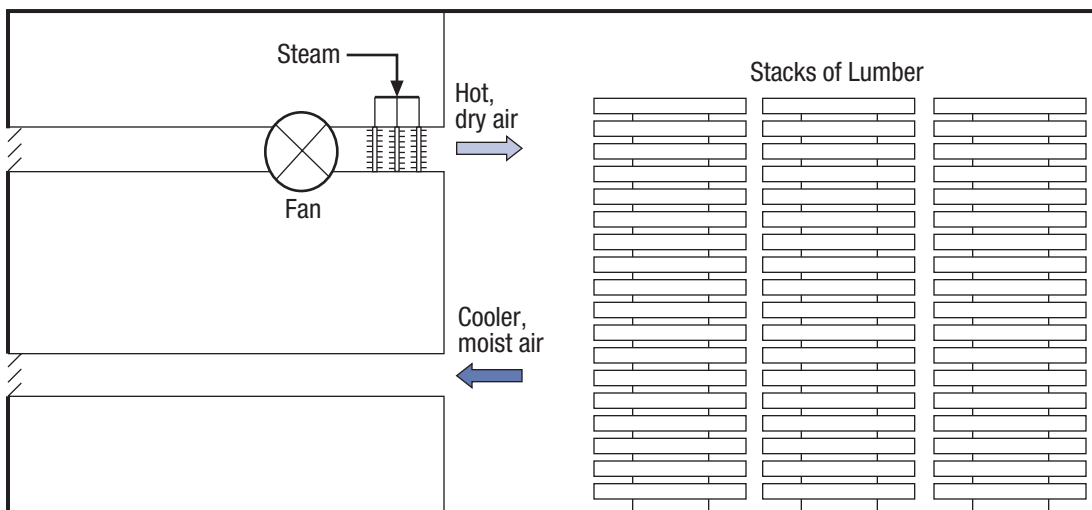
Figure 2.1a: Simplified Schematic of Steam-Heated Lumber-Drying Kiln
