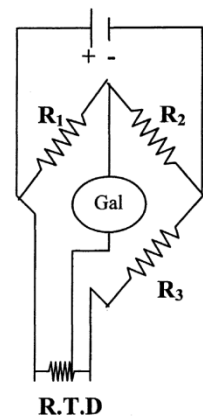
Three-wire R.T.D
