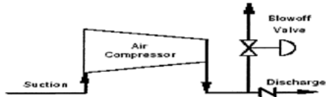
Air Compressor Anti-Surge Valve
