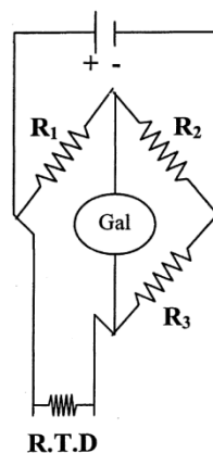
Two-wire R.T.D
