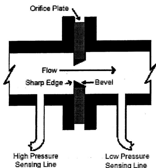
A Typical Orifice Plate
