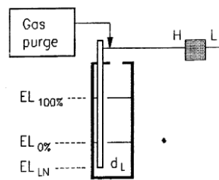
Arrangement-5: Open equipment; No reference leg; External gas purging (entry point near purge pipe); Terms T-1/3/4 = 0.
