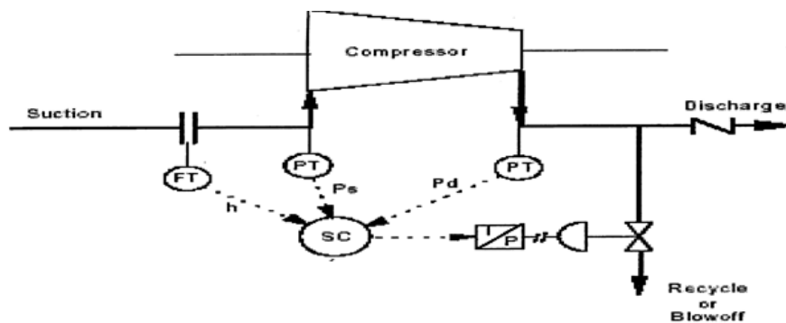
Pressure Ratio Method
