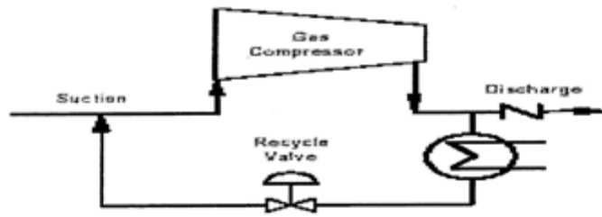
Gas Compressor Anti-Surge Valve
