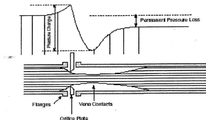
Orifice Plate Installation with Pressure Profile
