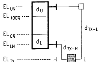
Arrangement-2: Closed equipment; Wet reference leg.
