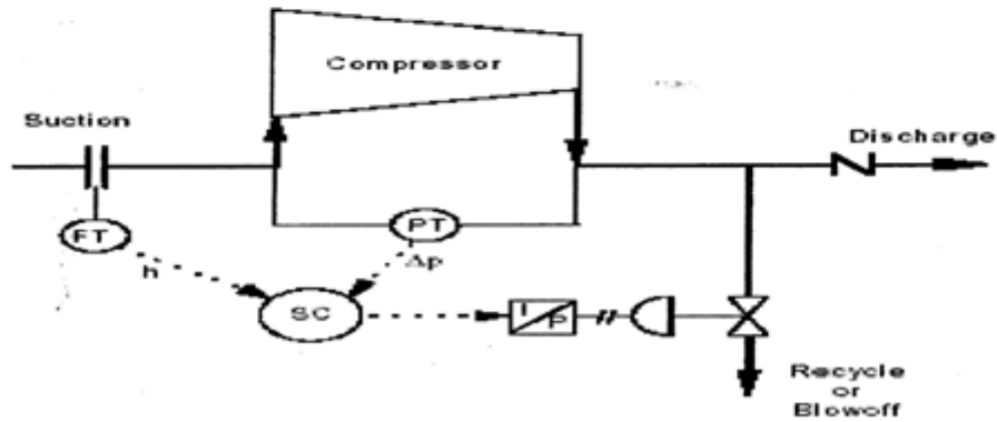
Pressure Rise Method
