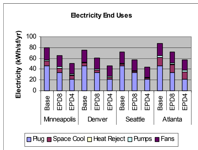
Figure 2.41 Electricity end uses for the base case and lower plug loads of 8 W/sf (EPD8) and 4 W/sf (EPD4).
