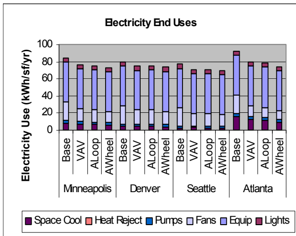
Figure 2.45 Electricity end uses for the base case, VAV system (VAV), and the advanced case with a run-around loop (ALoop) and an enthalpy wheel (AWheel).
