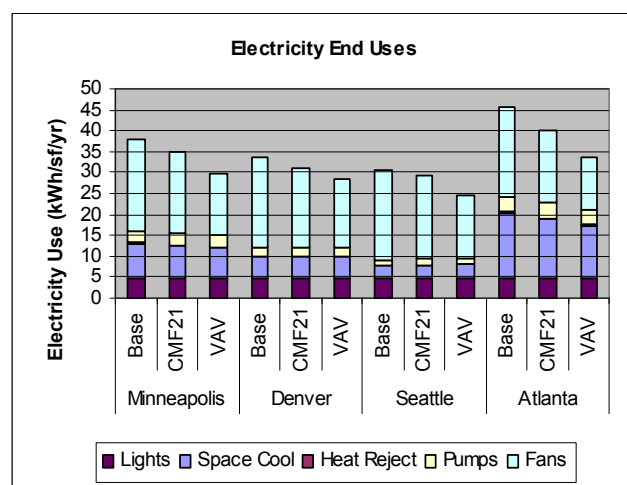
Figure 2.1 Electricity end uses for the three cases.
