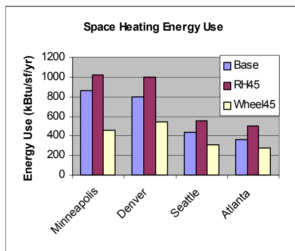
Figure 2.36 Space heating energy use for the base case, relative humidity controls of 40% and 50% (RH45), and enthalpy wheel with tighter humidity controls (Wheel45).
