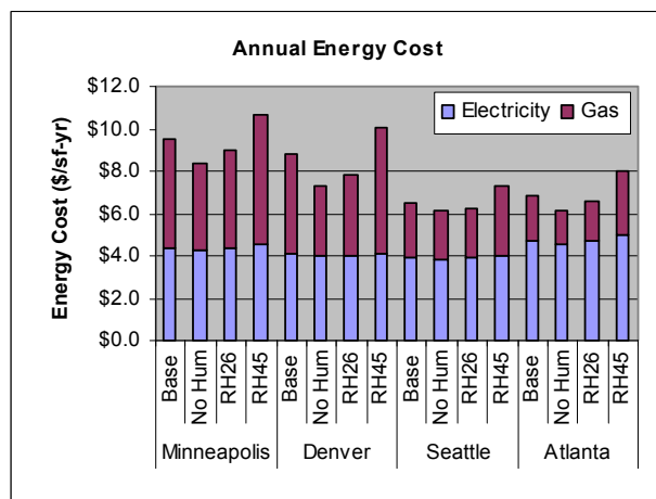
Figure 2.34 Annual energy costs for the base case, no humidity controls (NoHum), minimum RH of 20% and maximum RH of 60% (RH26), and minimum RH of 40% and maximum RH of 50% (RH45).
