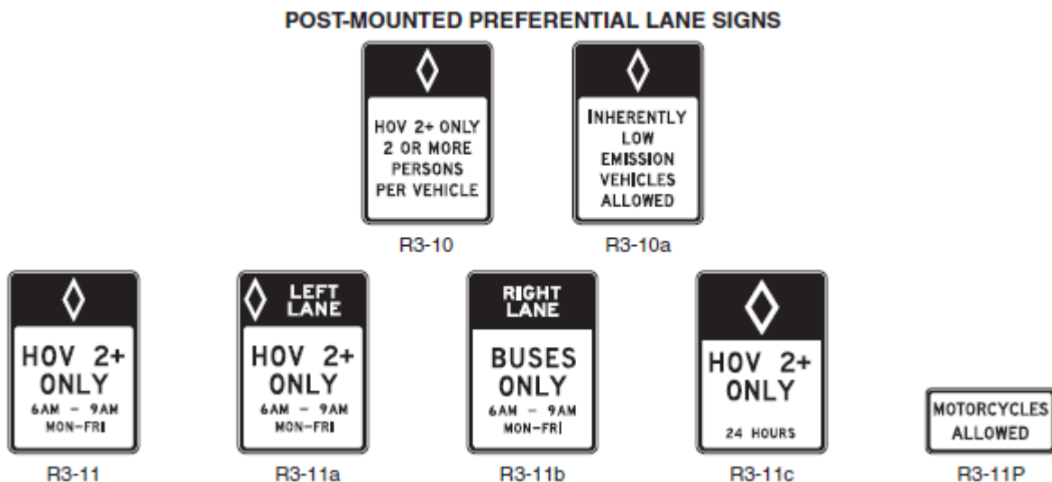
Figure 2G-1. Preferential Lane Regulatory Signs and Plaques (Sheet 1 of 2)
