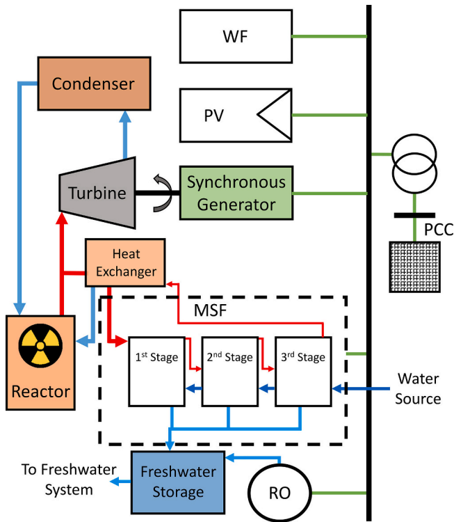
Fig. 1. Considered HyPP layout.
