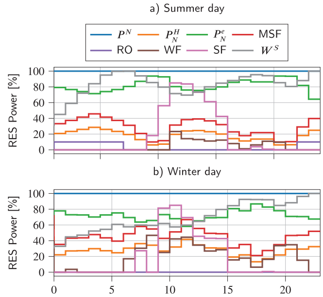
Fig. 8. Study Case A: Operational Summary.
