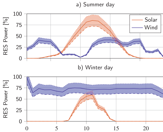
Fig. 7. Solar and wind resources.
