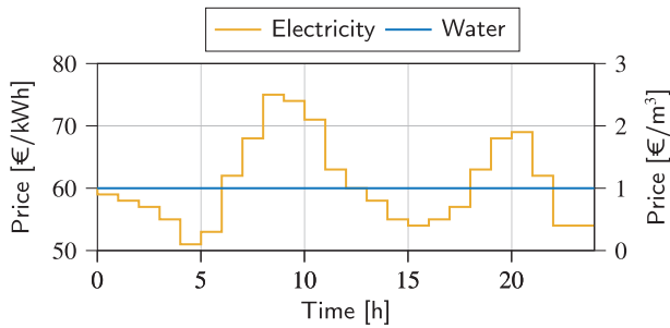
Fig. 6. Electricity and water prices.
