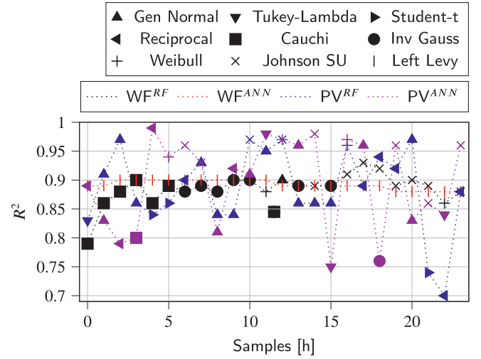
Fig. 4. Error distribution per method and resource.
