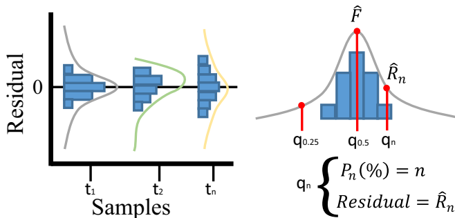
Fig. 3. Residual distribution characterisation concept.
