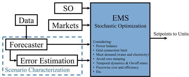
Fig. 2. Concept of a data-driven stochastic EMS.
