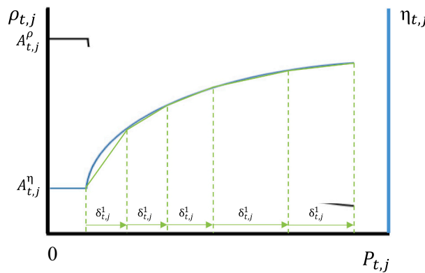
Fig. 9. Piecewise linear cost and efficiency representation.
