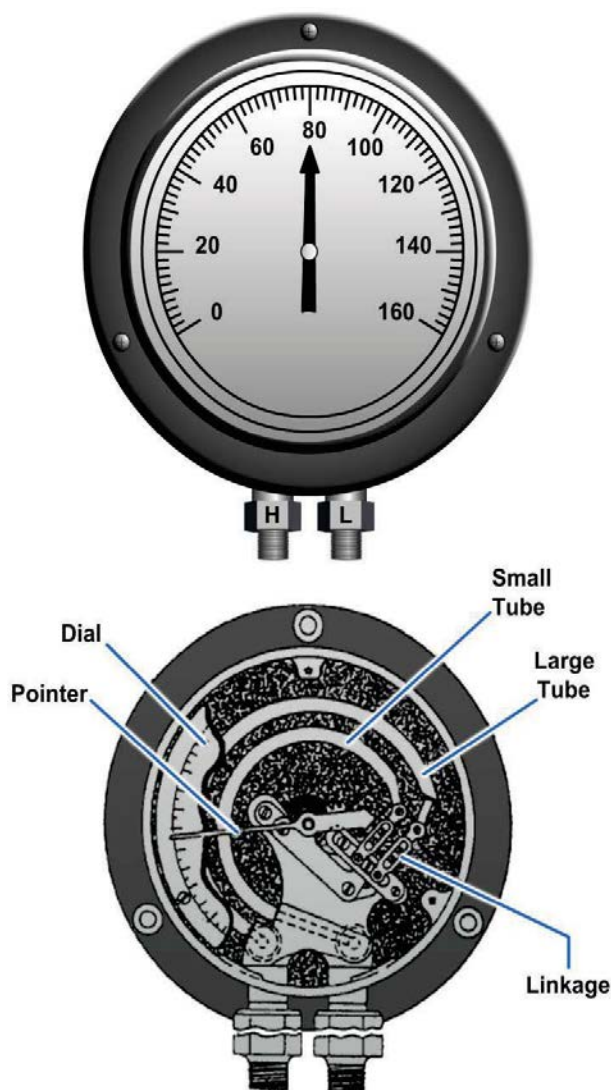
Figure 11-6 — Bourdon-tube differential pressure gauge.
