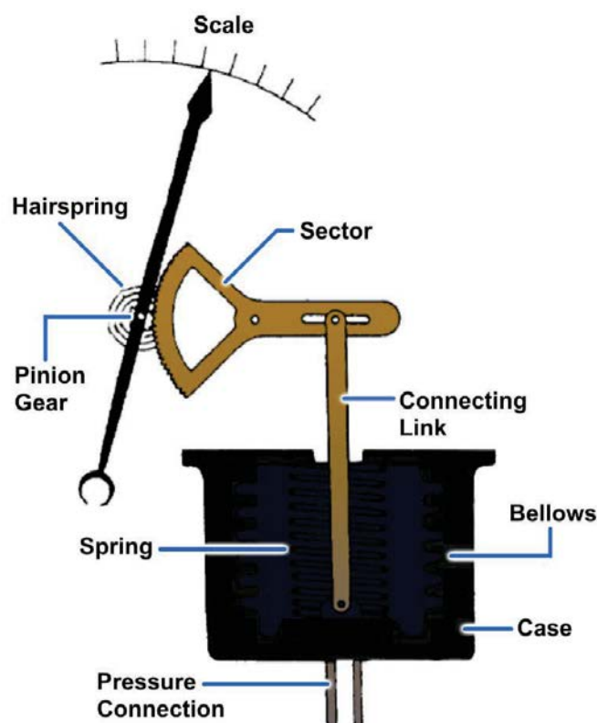
Figure 11-7 — Bellows gauge.
