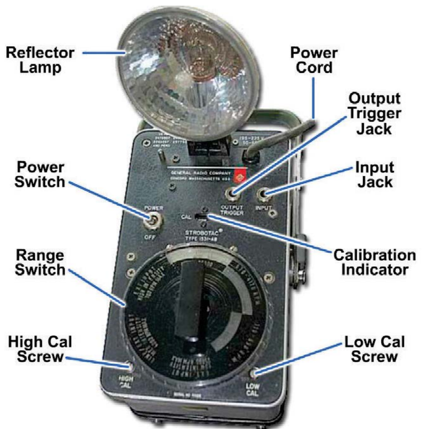
Figure 11-24 — stroboscope tachometer.
