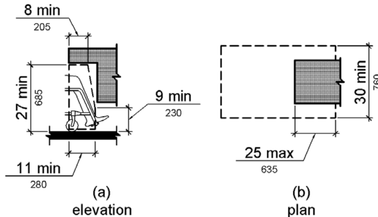
Figure 306.3 Knee Clearance
