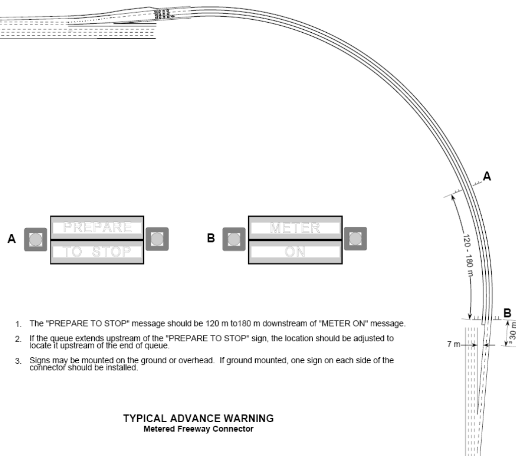
Figure 10-14: Typical Advance Warning Signing Layout 28
