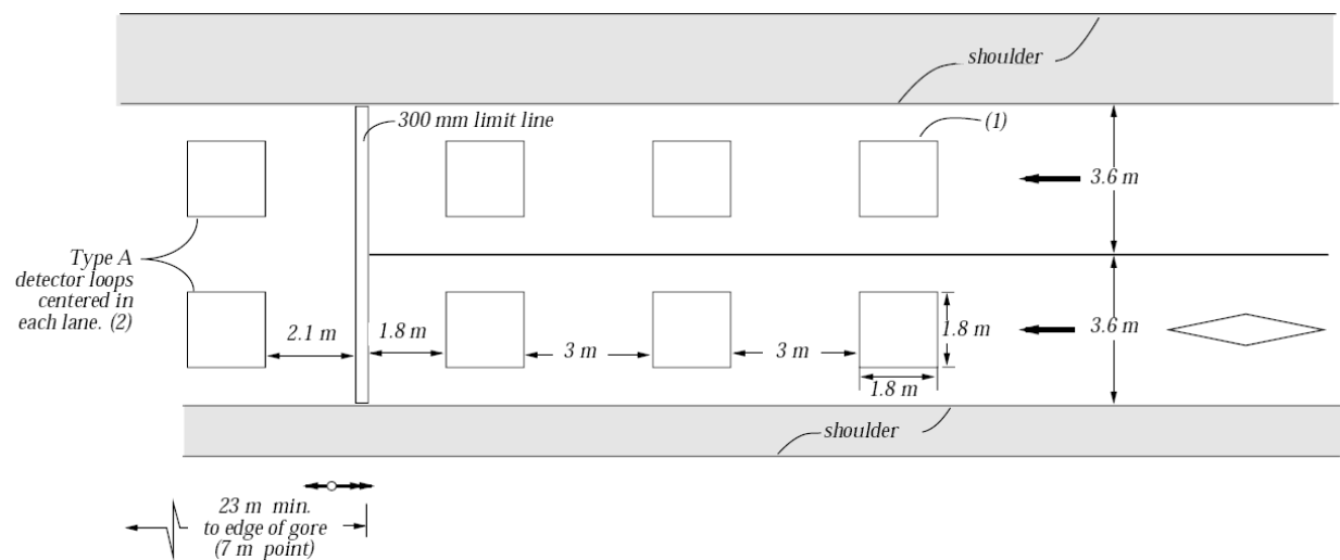
Figure 10-9: Typical Passage and Demand Detector Layout (Two Lane Ramp) 28
