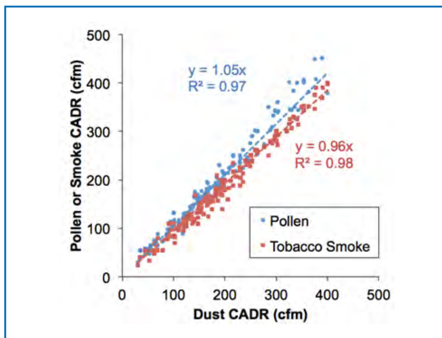
Figure 9. Comparison of CDRs for pollen, dust, and tobacco smoke particles for over 350 air cleaners tested and reported on the AHAM website: www.ahamdir.com/aham_cm/site/pages/index.html .
