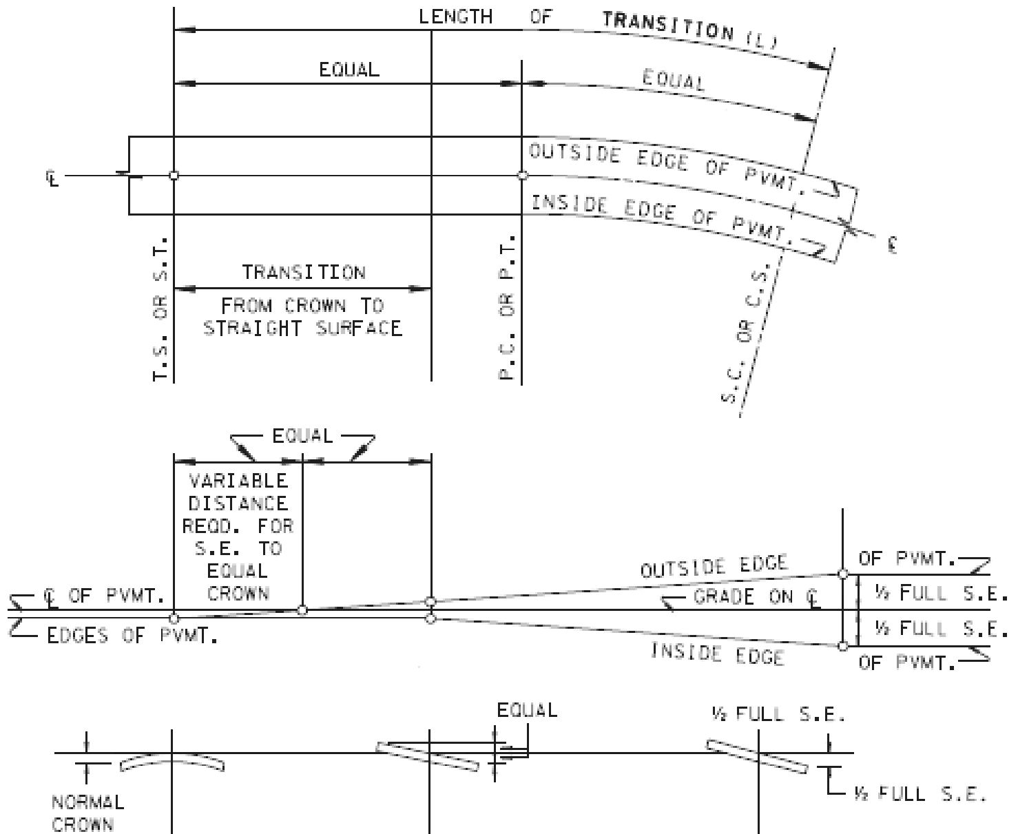
Typical Superelevation Transition 2-Lane Roadway
