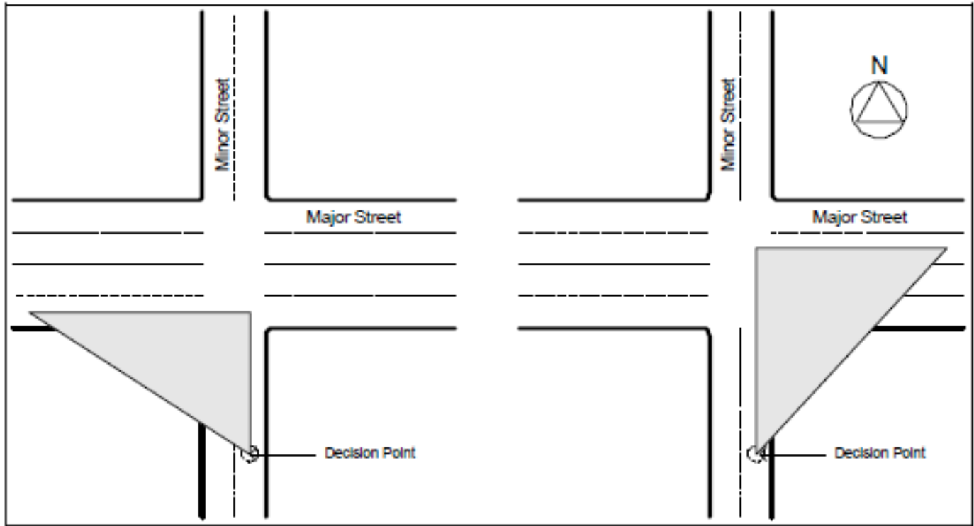
Figure 4.1. Approach Sight Triangles
