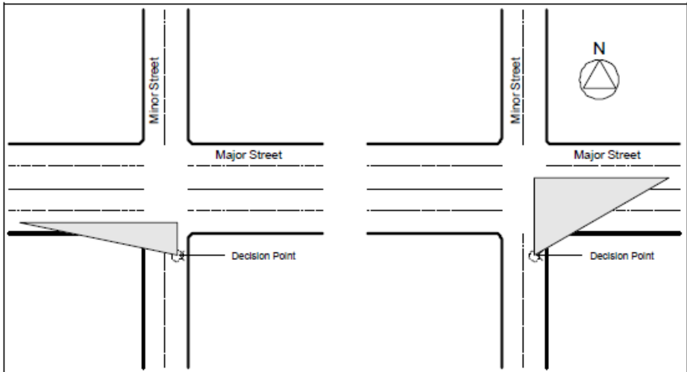
Figure 4.2. Departure Sight Triangles
