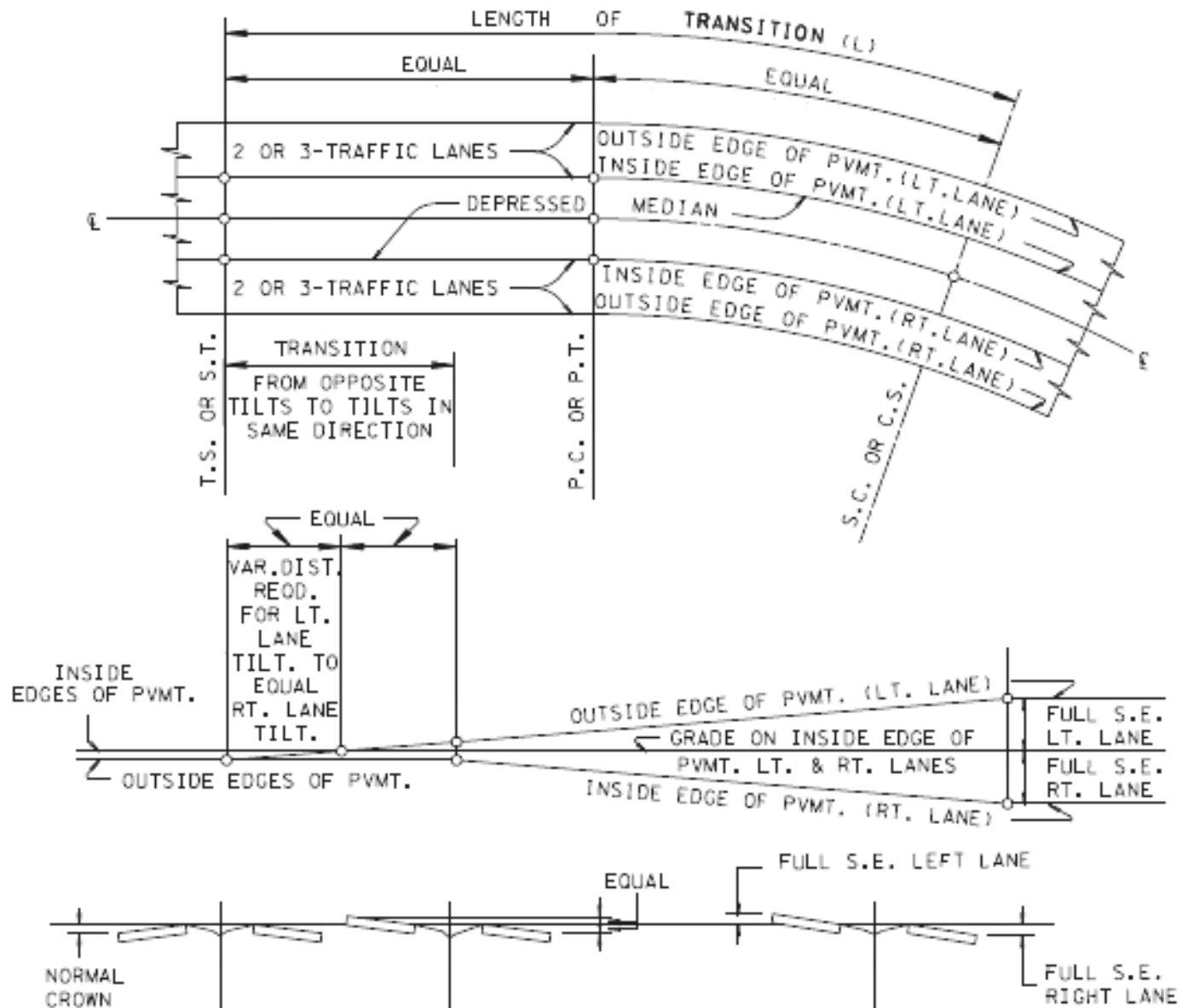
Typical Superelevation Transition Roadway With Depressed Median
