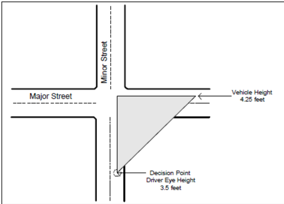
Figure 4.3. Heights Pertaining to Sight Triangles
