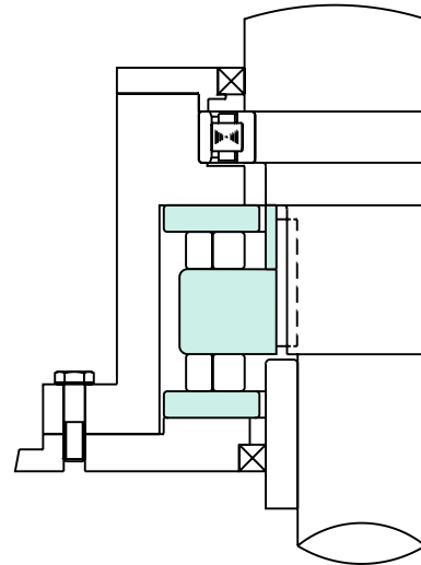
Double Acting Thrust
