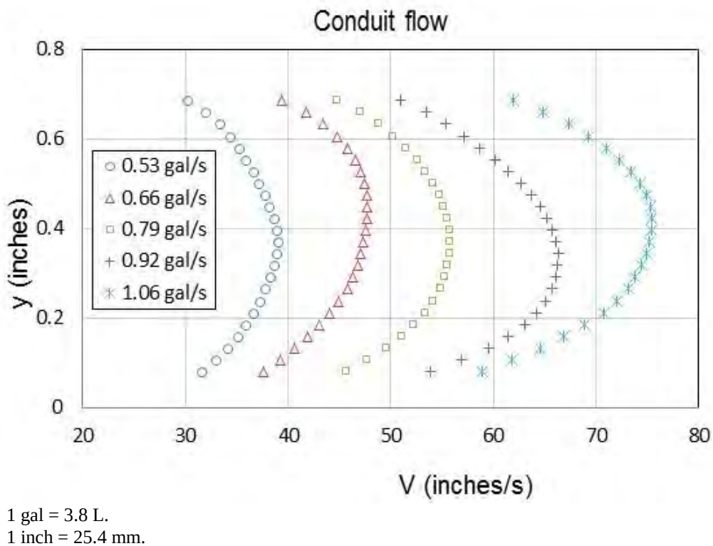
Figure 19. Graph. Velocity profiles of conduit flow with P220 sandpaper bed.
