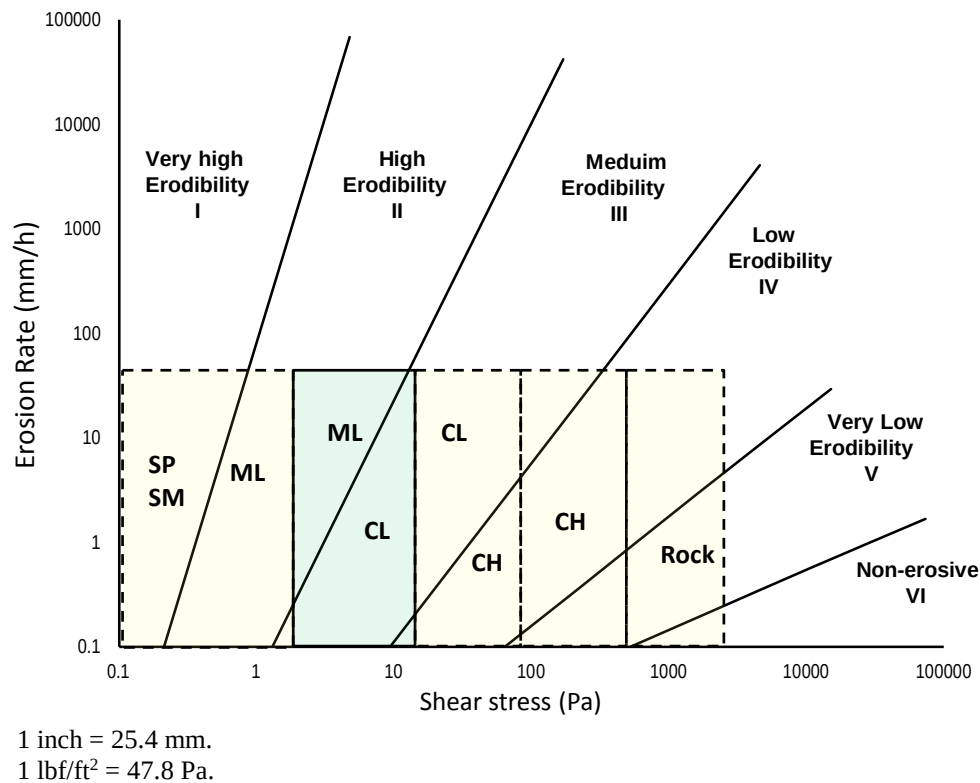
Figure 2. Graph. Division of materials into zones for specific devices.
