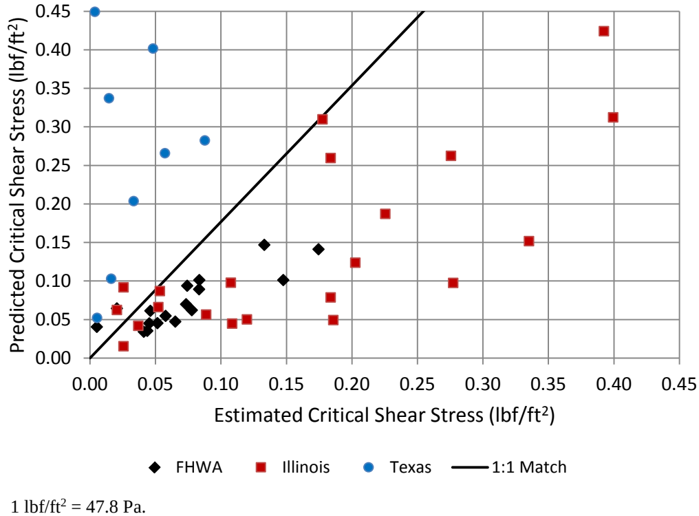
Figure 57. Graph. Critical shear stress comparison with FHWA, Illinois, and Texas data.
