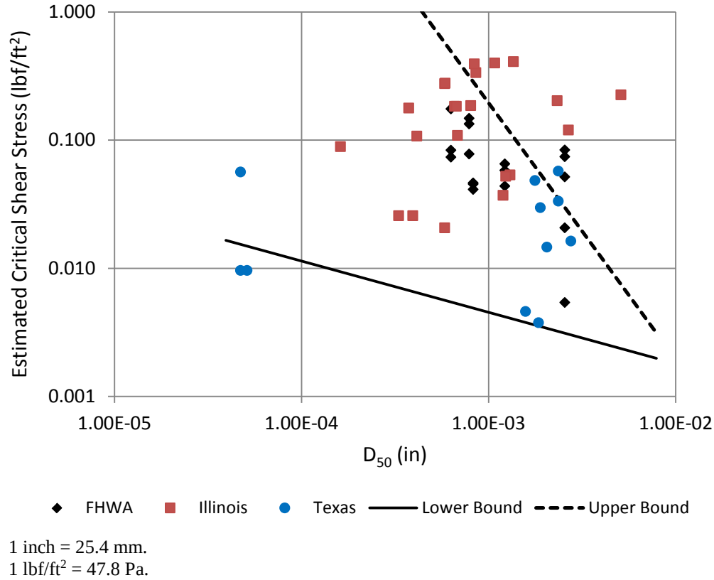
Figure 51. Graph. Comparison of critical shear stress with Briaud bounds.
