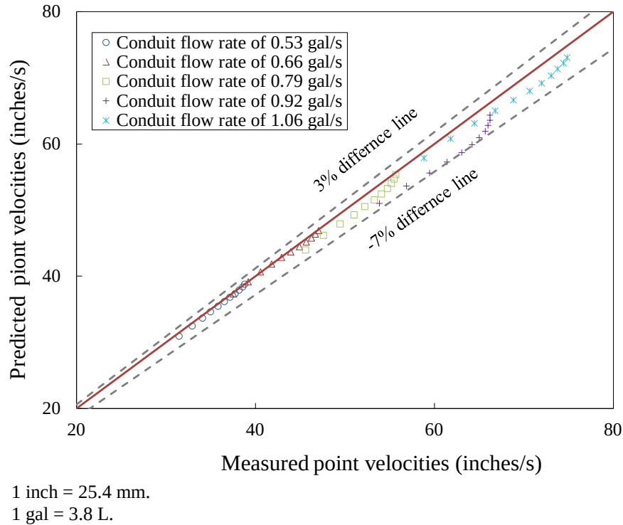
Figure 30. Graph. Comparison of conduit flow point velocities on a P220 sandpaper bed.
