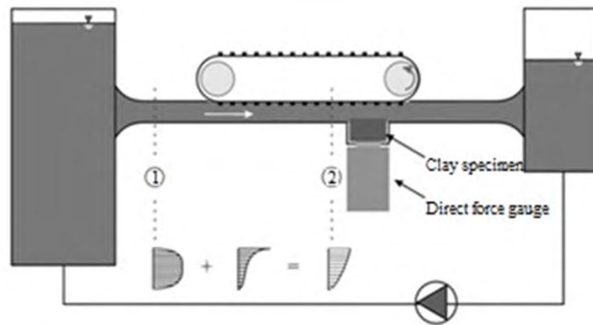
Figure 12. Diagram. Schematic of the ESTD.
