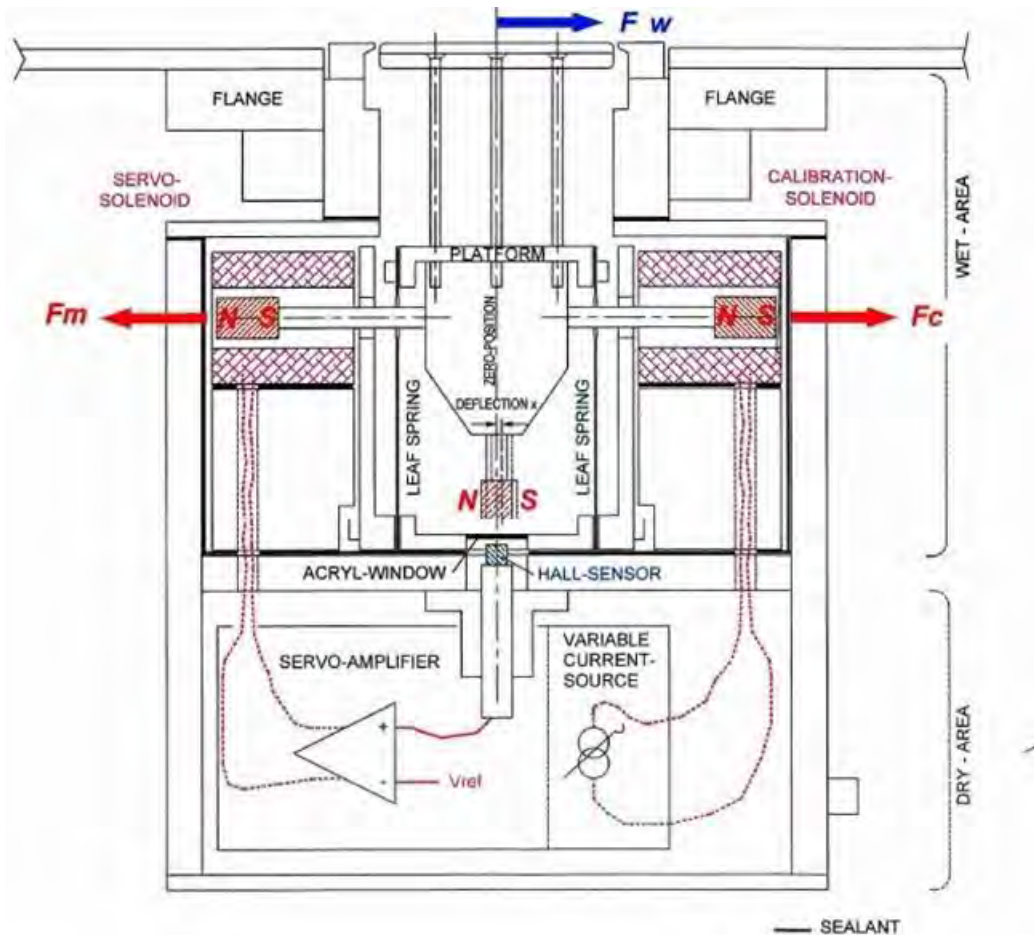
Figure 14. Diagram. Principles of force measurements in the horizontal direction.
