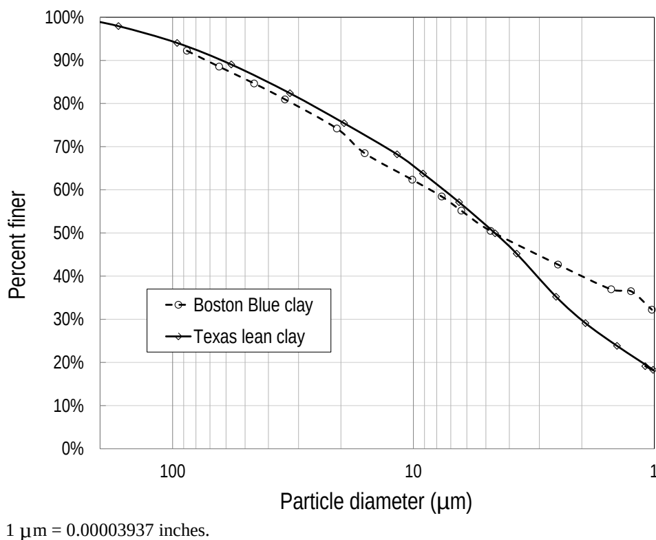
Figure 36. Graph. Gradation of compacted clays.
