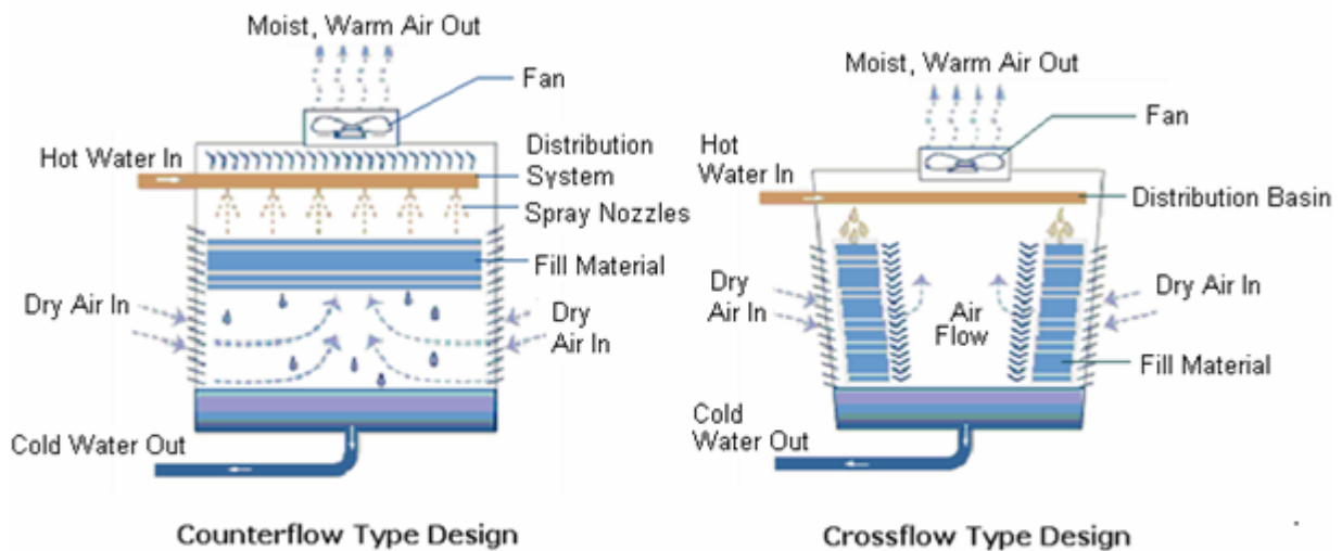
FIGURE - 11 TYPES OF COOLING TOWER
