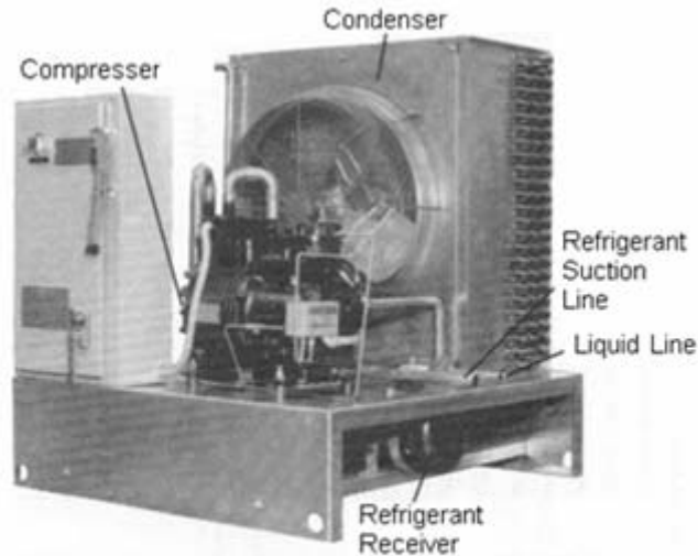
FIGURE - 8 AIR COOLED CONDENSING UNIT
