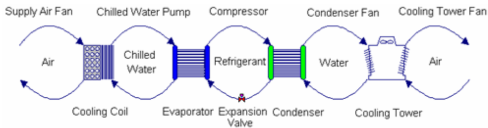
FIGURE - 6 CHILLED WATER SYSTEM WITH WATER COOLED CONDENSER
