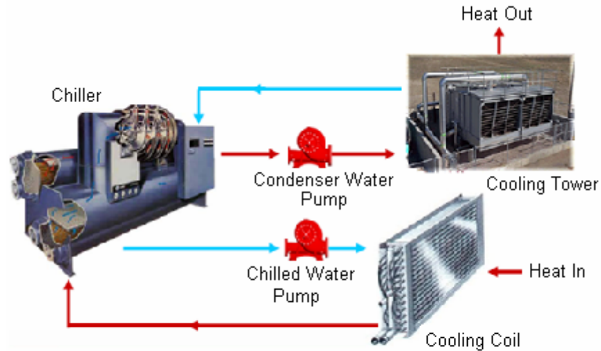
FIGURE - 4 CHILLED WATER SYSTEM
