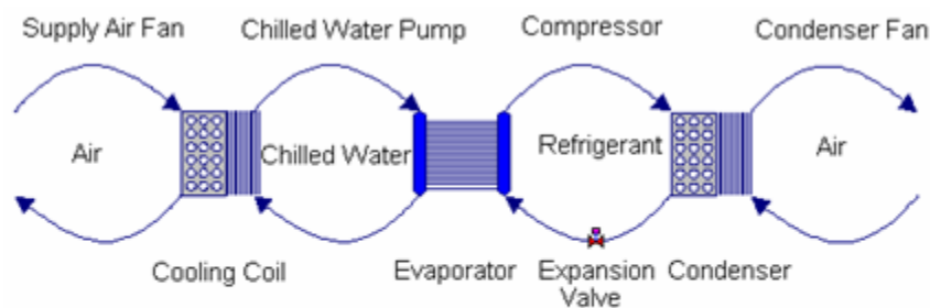
FIGURE - 5 CHILLED WATER SYSTEM WITH AIR COOLED CONDENSER
