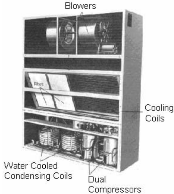
FIGURE - 3 PACKAGED AIR CONDITIONER UNITS
