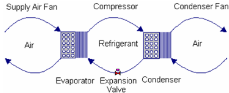
FIGURE - 1 DX SYSTEM
