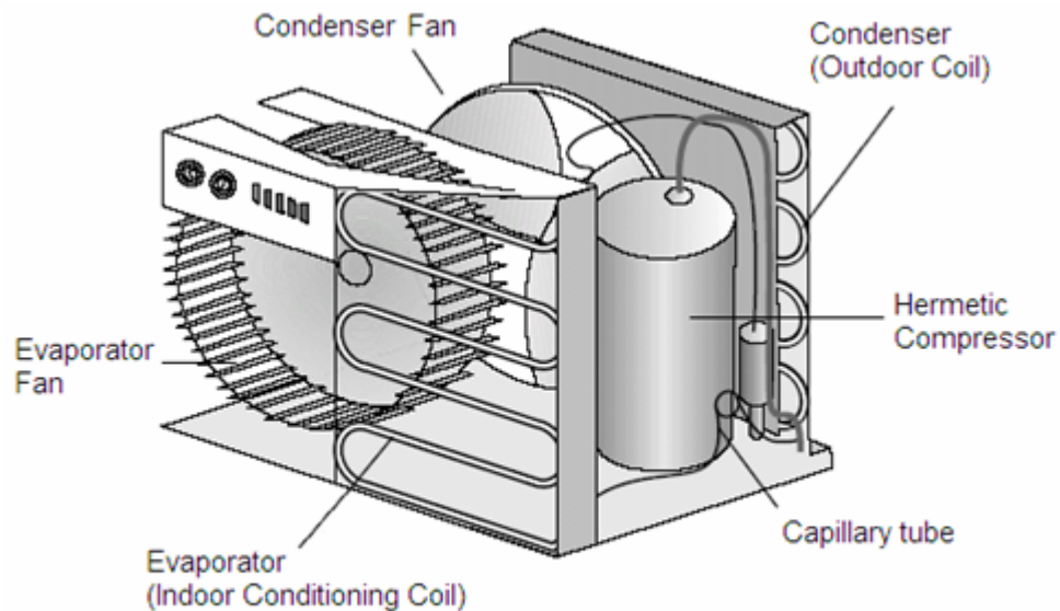
FIGURE - 2 TYPICAL ROOM AIR CONDITIONER
