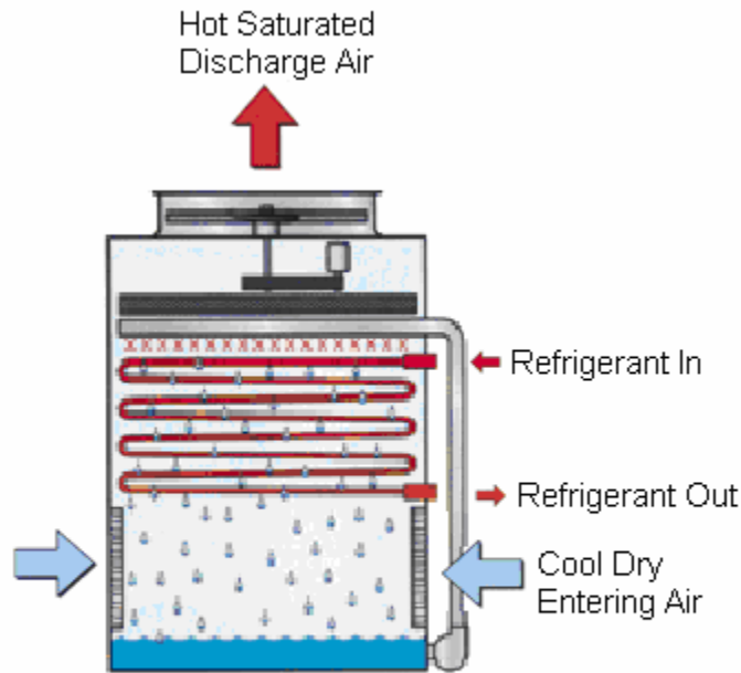
FIGURE - 10 EVAPORATIVE CONDENSER
