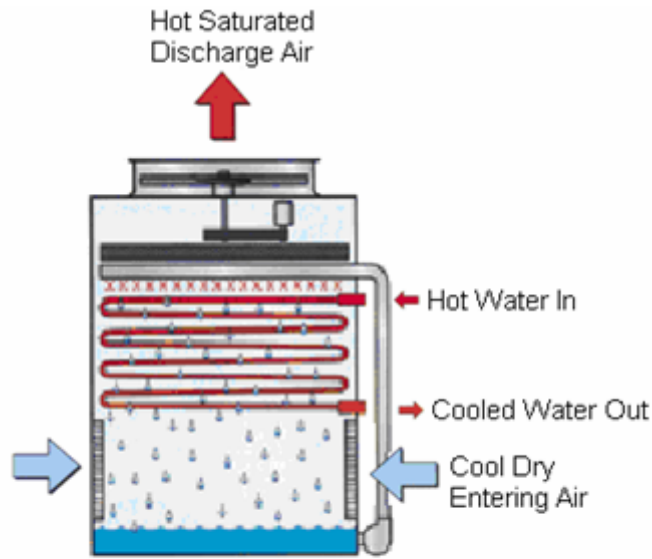
FIGURE - 9 CLOSED CIRCUIT COOLER
