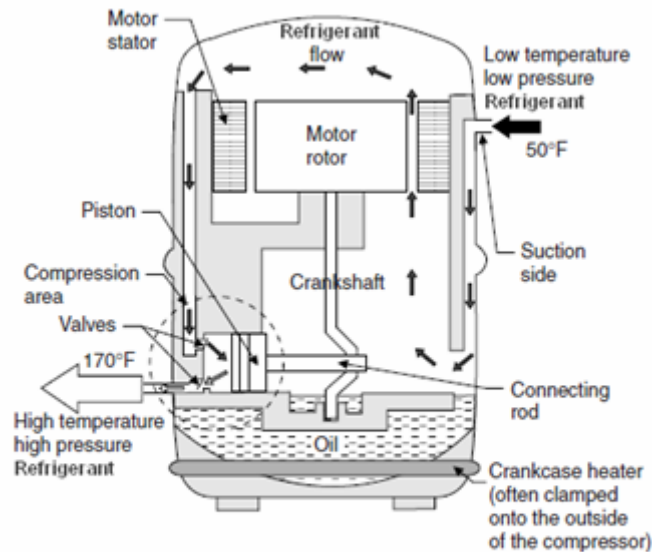
FIGURE - 7 CROSS SECTION OF HERMETIC COMPRESSOR
