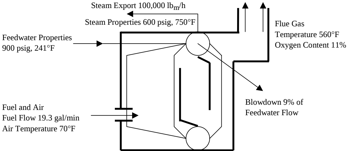
Fig. 1. Example boiler.
