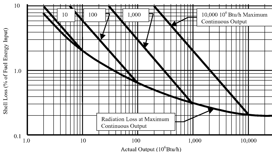
Fig. 4. ABMA typical shell loss.
