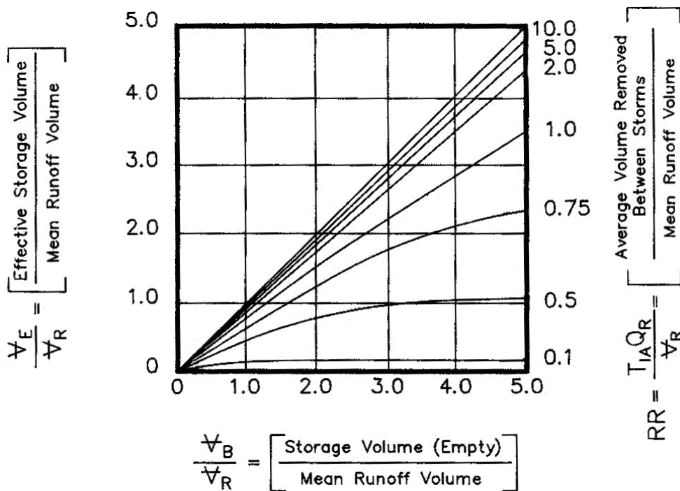
Figure 3-1 Ratio of Effective Storage Volume to Mean Runoff Volume (modified after Driscoll et al., 1986)
