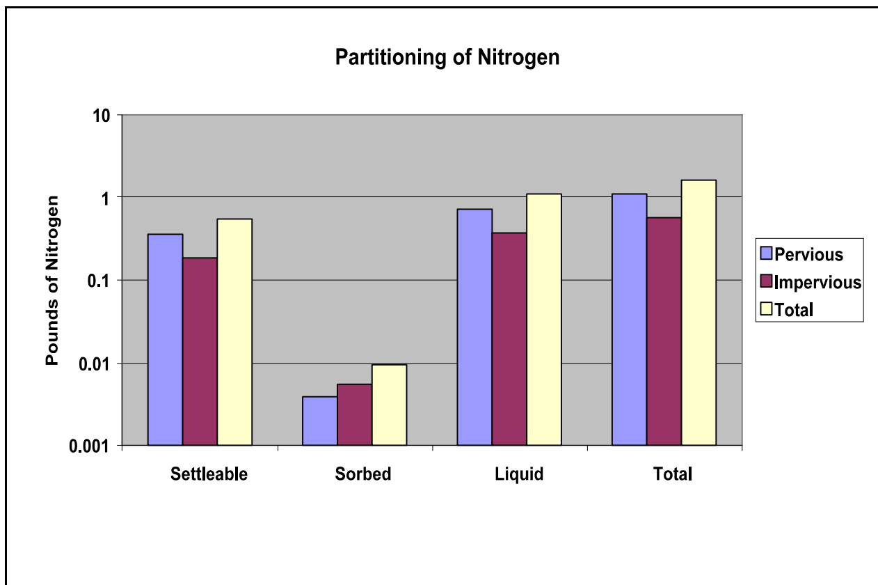
Figure 4-3 Nitrogen Partitioning
