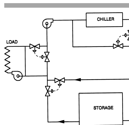
Figure 11. Typical encapsulated ice configuration. (d)
