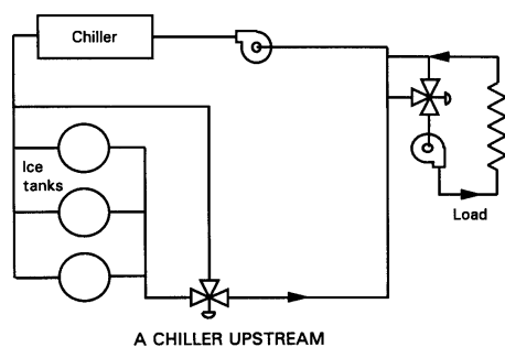
Figure 8. Typical internal-melt ice-on-coil configuration. (d)
