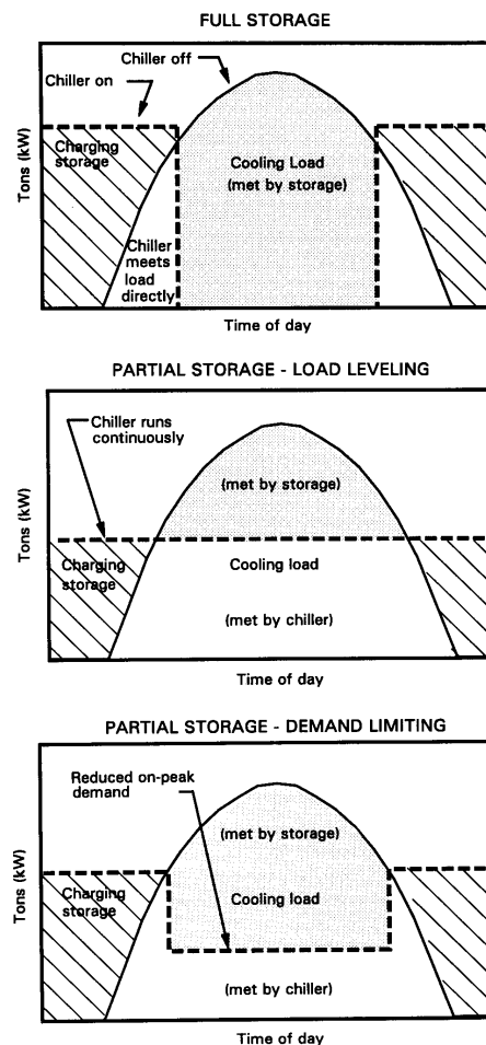
Figure 14. Cool storage design options. (e)
