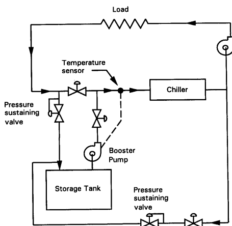
Figure 13. Typical eutectic salt configuration. (e)
