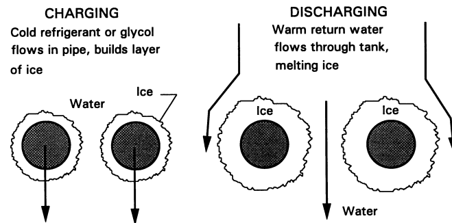
Figure 4. External-melt ice-on-coil. (b)
