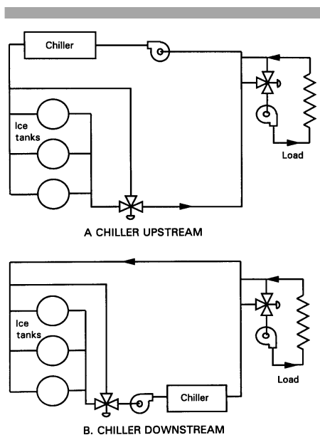
Figure 15. Upstream and downstream chiller configurations. (f)
