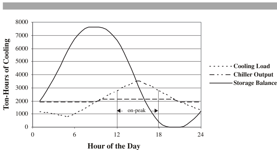
Figure 16. Chiller and storage sizing example.
