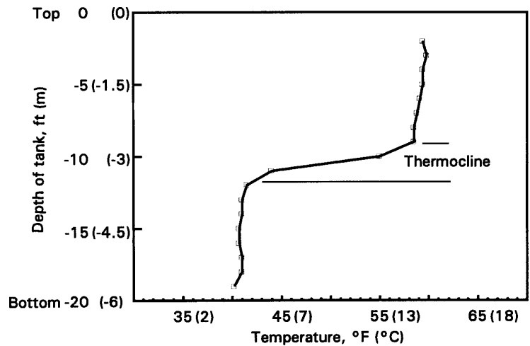
Figure 1. Chilled water stratification. (a)
