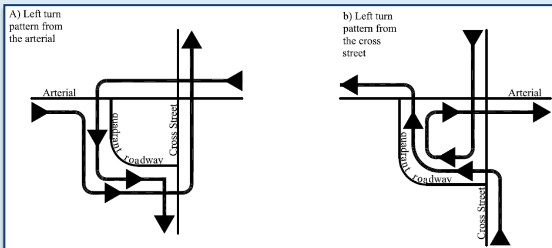
Figure 18. Schematic. The quadrant roadway (QR) intersection.
