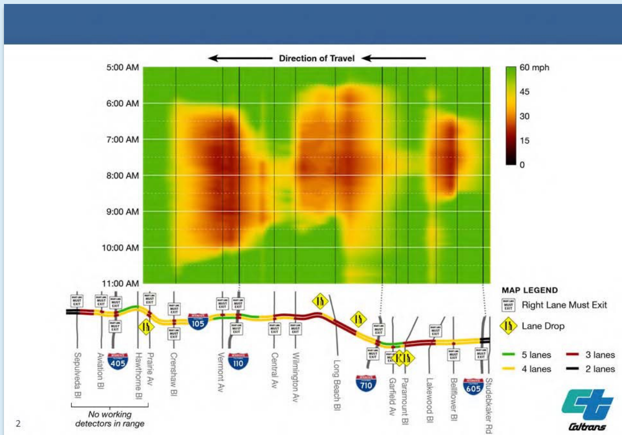
Figure 7. Graph. Speed contours over time and space showing bottleneck locations.
