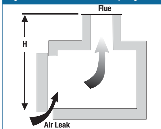
Figure 6. Air infiltration from furnace opening.
