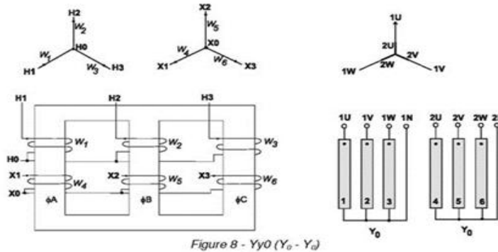
Figure 8 - Yy0 ( Y_0 - Y_0 )
