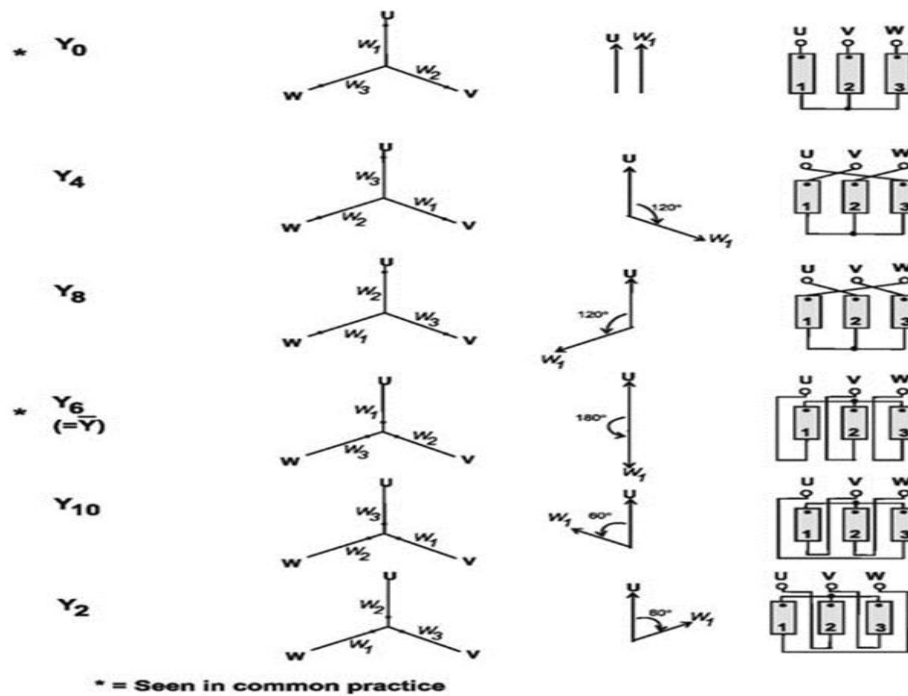
Six Ways to Wire a Wye Winding
