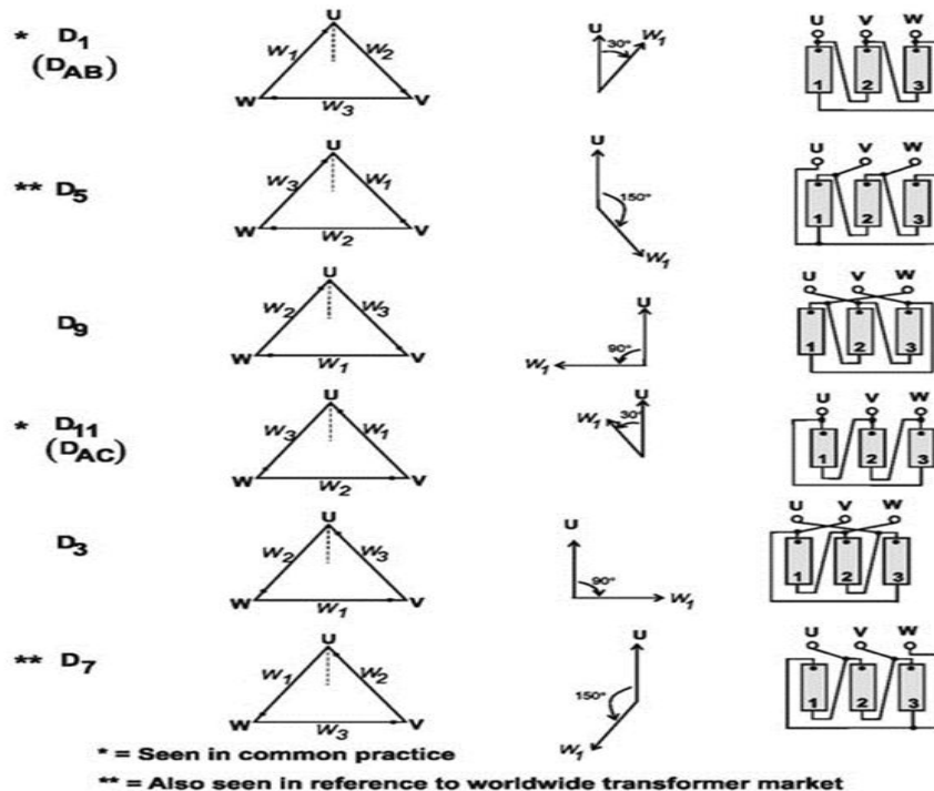
Six Ways to Wire a Delta Winding
