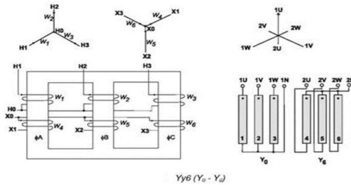
Yy6 ( Y_0 - Y_6 )
