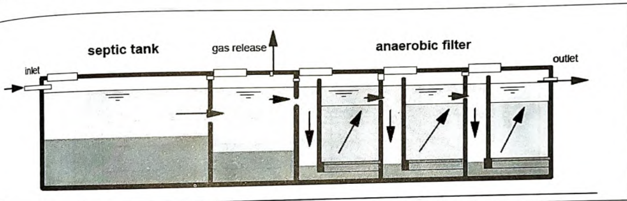
شكل (٤-٤) Anaerobic Filter
