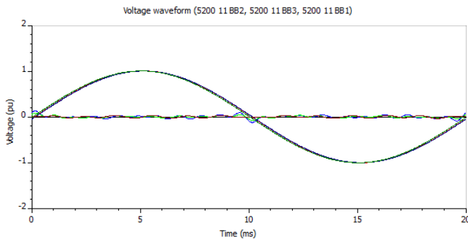
Fig. 15. Voltage waveform for PL Eagle 11 kV Bus and harmonic distortion.
