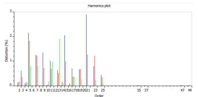
Fig. 14. Harmonics plot for Potline Eagle 11 kV Bus 1, 2 &amp; 3
