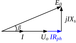
Fig. 7. Simplified voltage phasor diagram of the synchronous generator operating with resistive load R_N ( U_o = IR_N ).
