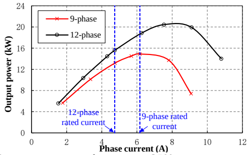
Fig. 16. Output power versus phase current @500 rpm.
