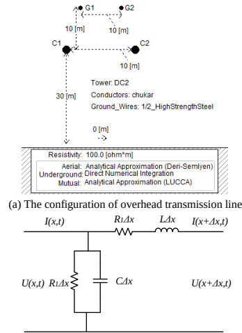
(a) The configuration of overhead transmission line
