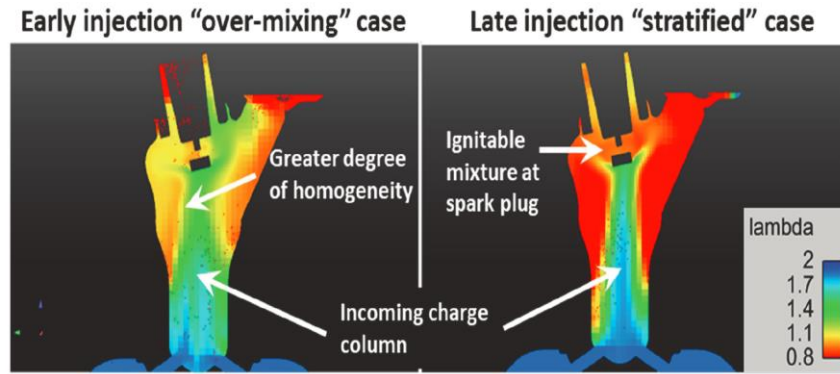
Figure 15. Mixture preparation with early (left) and late fuel injection (right) timing in the pre-chamber at the time of the spark with constant pre-chamber fuel quantity [42].
