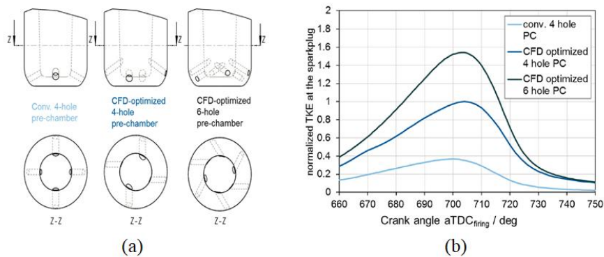
Figure 14. (a) Different pre-chamber designs and (b) the normalized turbulent kinetic energy at the spark plug [18].
