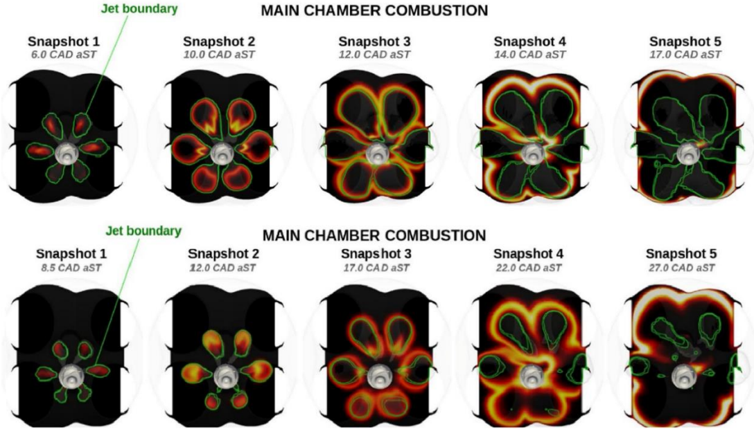
Figure 7. Visualization of the main chamber combustion at (top row) stoichiometric conditions and (bottom row) diluted conditions [49].
