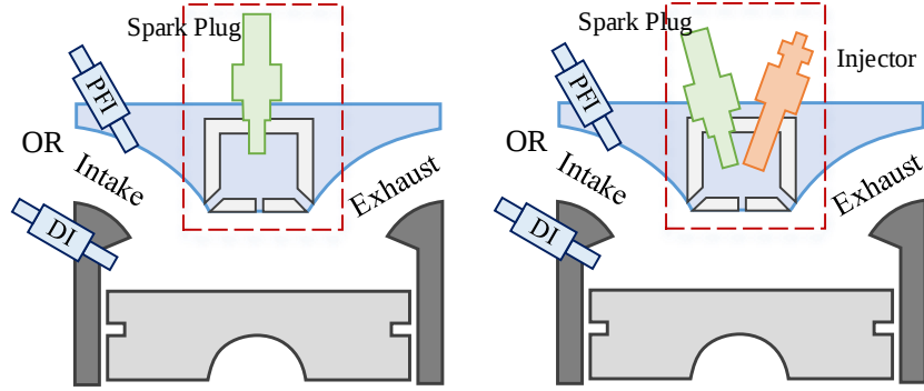
Figure 1. Configurations of passive (left) and active (right) pre-chamber ignition systems.
