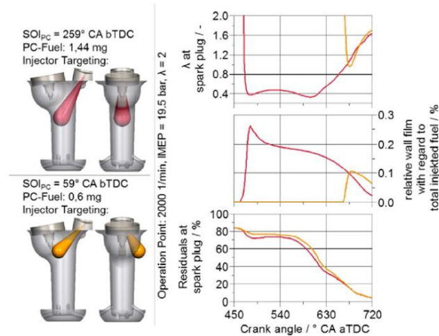
Figure 16. Comparison of different fuel injection strategies [12].
