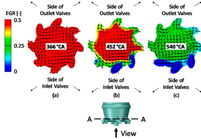
Figure 2. Scavenging across the pre-chamber during the intake stroke (EGR indicates the residual gas mass fraction) [40].
