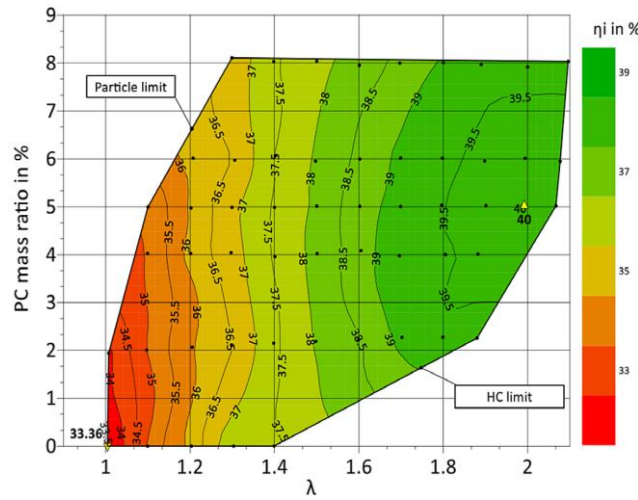
2 3 Figure 19. Contour map of the indicated efficiency map at IMEP of 6 bar @ 1500 rpm [33].
