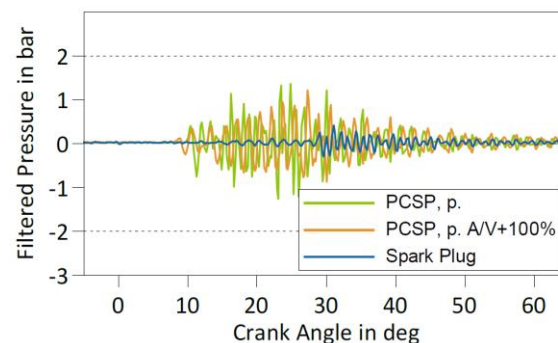
Figure 10. Comparison of filtered pressure traces between the conventional spark ignition and the pre-chamber ignition at BMEP of 16 bar @ 2000 rpm [75].
