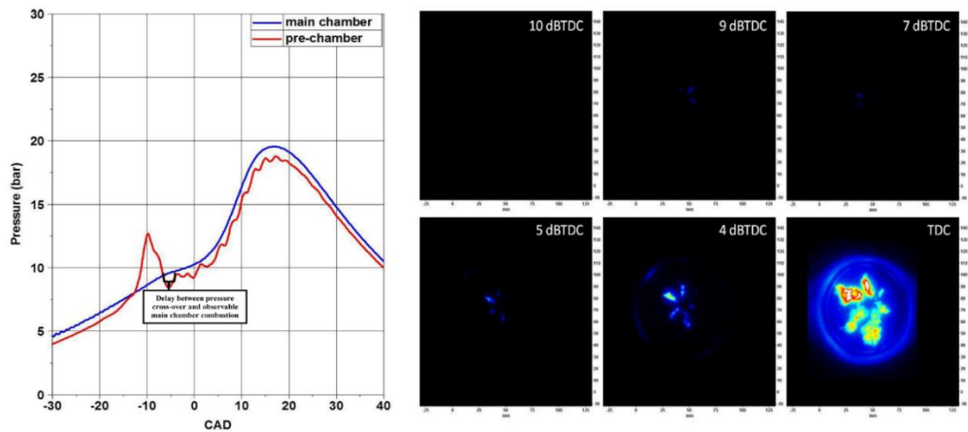
Figure 5. Pressure traces (left) and visualizations (right) during jet ejection processes on an optical engine [60].
