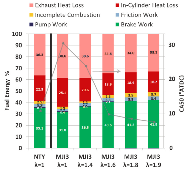
Figure 20. Comparison of efficiency loss pathways between the SI (NTY) and TJI (MJI3) at a knock limited condition (12 bar BMEP @ 3000 rpm) [42].
