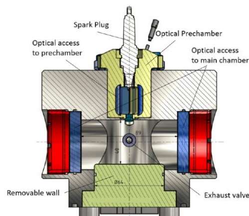
18 19 Figure 17. Schematic of the optical pre-chamber [67].
