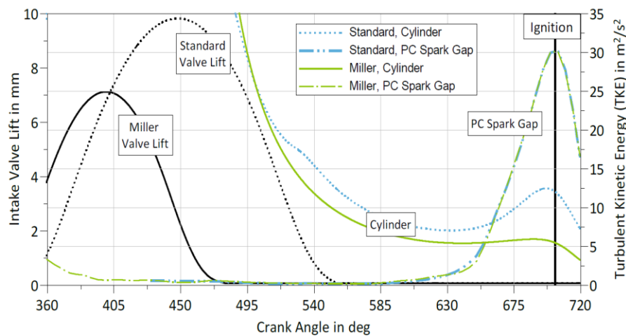
Figure 22. Comparisons of averaged turbulent kinetic energy levels in the cylinder and around the pre-chamber spark gap with standard and Miller camshafts at the BMEP of 4 bar @ 1250 rpm [75].
