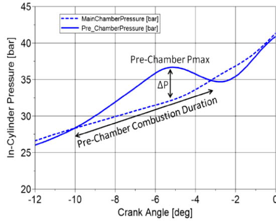
Figure 4. Pre-chamber combustion duration indicated by pressure traces in the pre-chamber and the main chamber [50].
