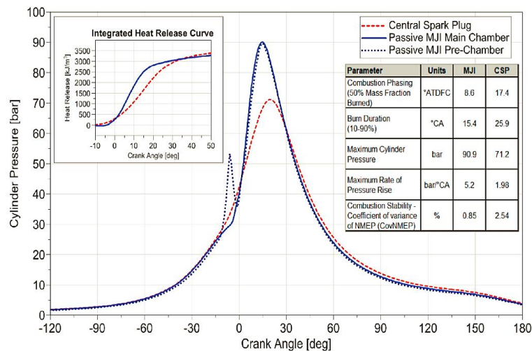
Figure 9. Comparison of the combustion profile between the passive TJI and the conventional SI at BMEP of 18 bar @ 4000 rpm [42].
