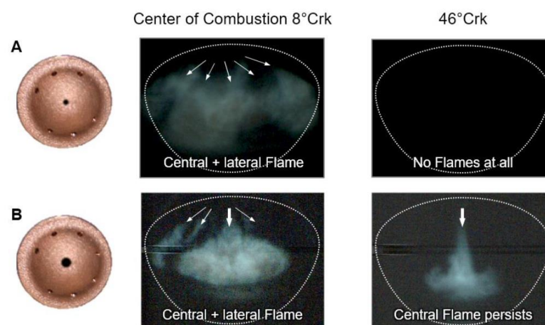
21 Figure 23. Optical images of two different pre-chamber layouts adopted on a single-cylinder 22 engine operating at the BMEP of 2 bar @ 1250 rpm [75].
