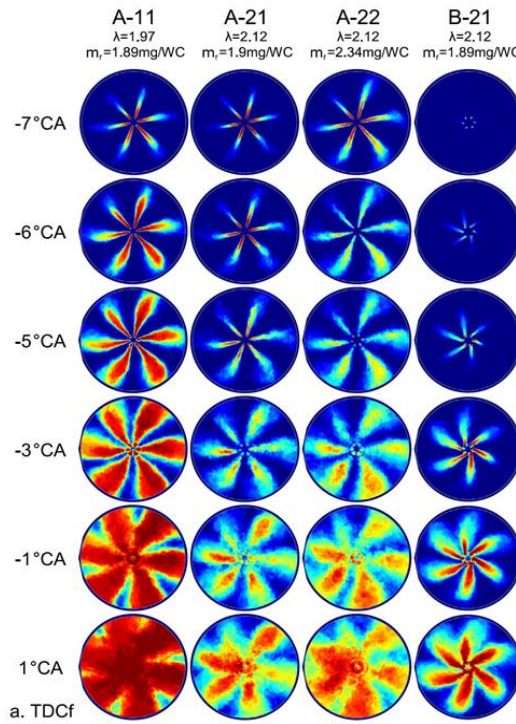
17 18 Figure 8. Comparison of averaged flame probability distributions in four cases [72].
