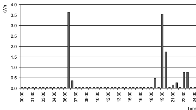
Fig. 3. Time Profile of Energy Use for the Professional Couple
