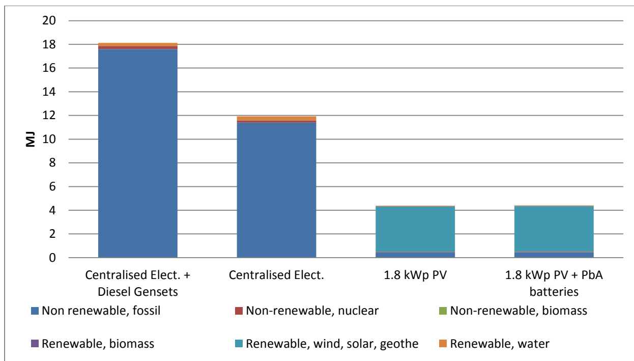
Figure 5. Cumulative Energy Demand of the four systems per 1 kWh (Method: Cumulative Energy Demand V1.08/Cumulative energy demand/Single score)
