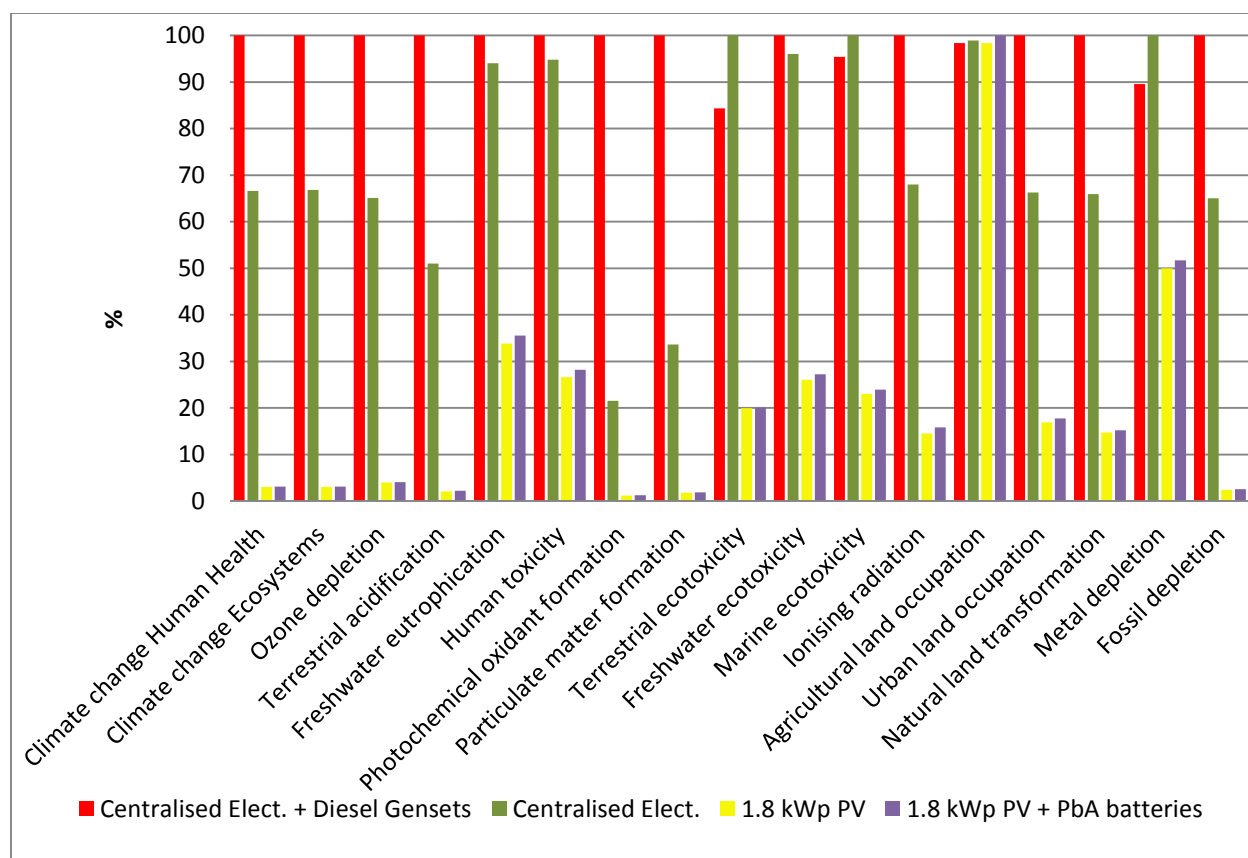
Figure 3. Characterised impacts of the Lebanese electricity with and without diesel gensets, and of a PV system (with and without battery), per 1 kWh of delivered electricity (Method: Recipe Endpoint (E) v1.07/WorldReCiPe E/E/Characterisation)
