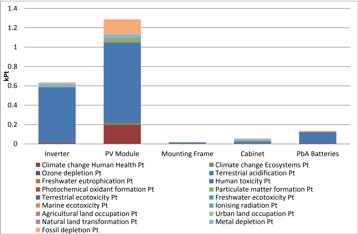
Figure 2. Single score impact assessment results (Method: Recipe Endpoint (E) v1.07/World ReCiPe E/E/Single Score)
