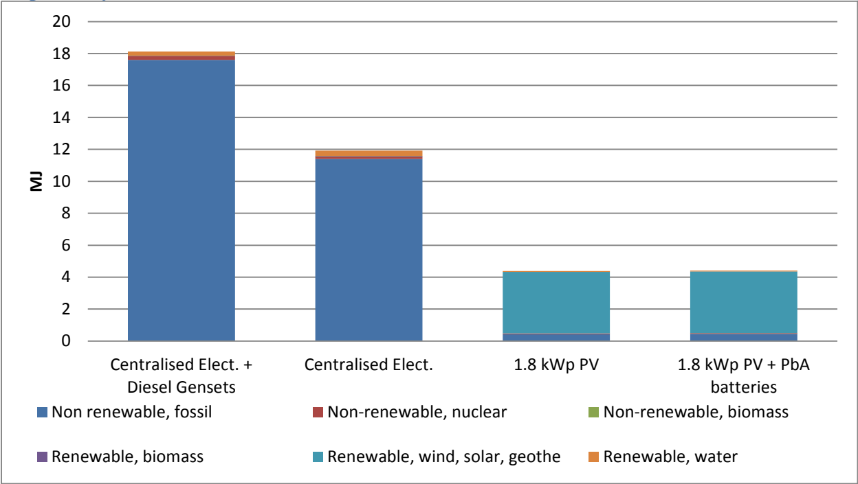
Figure 5). Consequently the gross energy requirement (GER), which is the life cycle primary energy inputs required to deliver a good or service to the point of interest (in the case of this study: 1 kWh) are summarised in Table 5.
