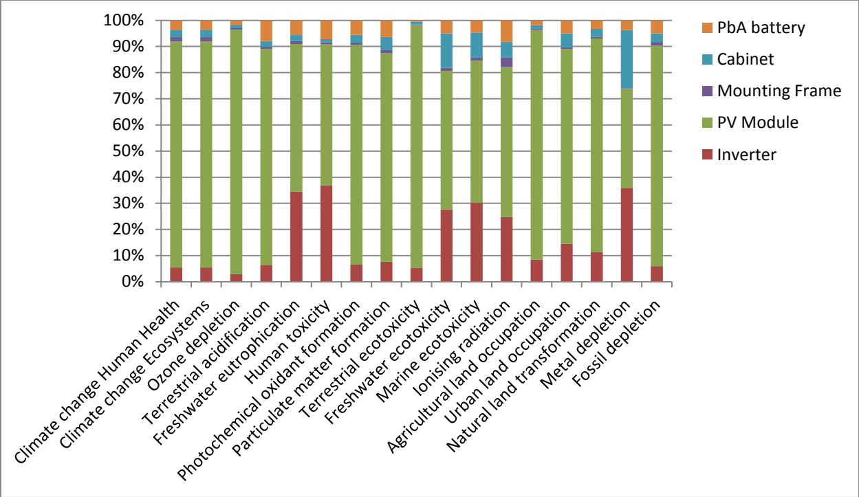
Figure 1. Characterised results of the photovoltaic system (Method: RecipeEndpoint(E) V1.07/WorldReCiPe E/E/Characterisation)
