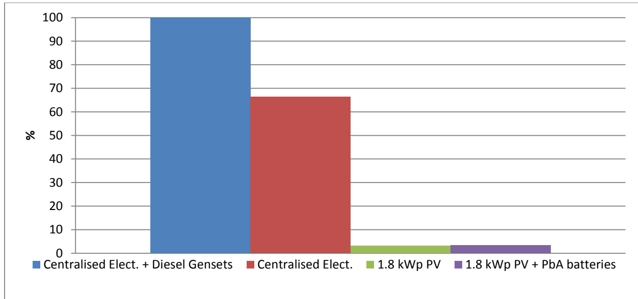
Figure 4. The attribute of CO 2 reduction of centralized Lebanese electricity generation and the PV cases (IPCC 2007 100aV1.02/Characterisation)
