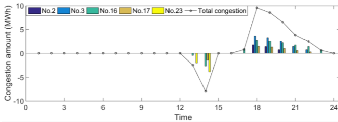
Fig.5. The system congestion and the branch congestion over daytime
