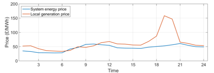
Fig.4. The price signal from system energy and the local generator
