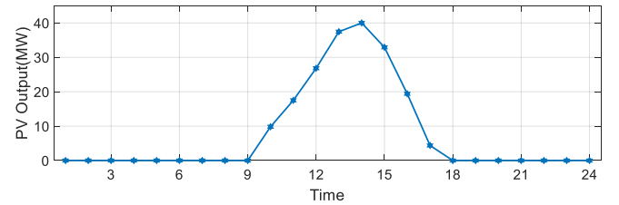
Fig.3. A daily PV output curve.
