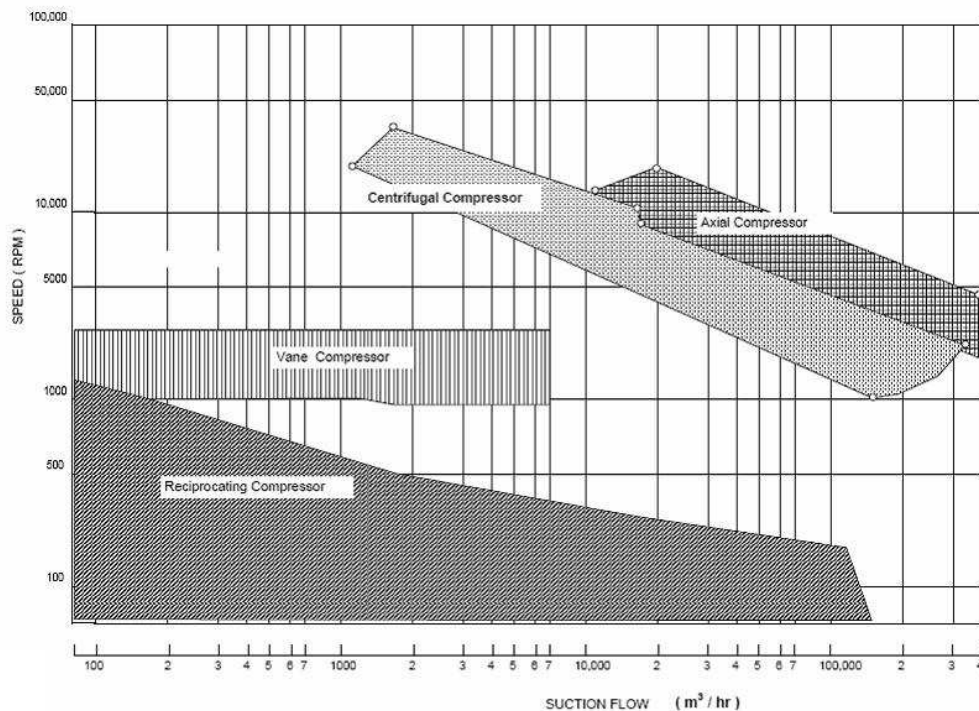
Fig. 4. Operating range of centrifugal compressor compared with other types of compressors
