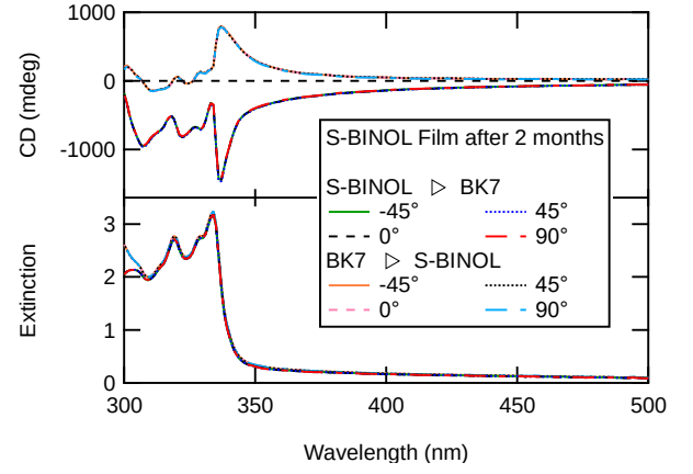
Figure 8. Extinction and CD of S-BINOL film for different rotational angles around the surface normal 2 months after evaporation. Note that curves of same propagation direction overlay.
