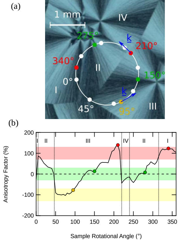
Figure 7. (a) Cross polarization picture of a R-BINOL film with the laser beam path during anisotropy factor measurements while the sample rotates around surface normal. (b) Related second order anisotropy factor at 400 nm SH for R-BINOL film at according sample rotational angle.
