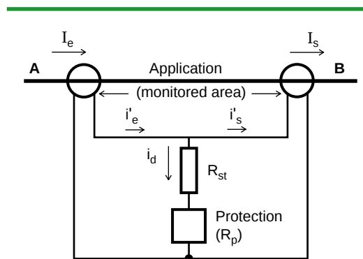
Fig. 21 : high impedance differential principle.
