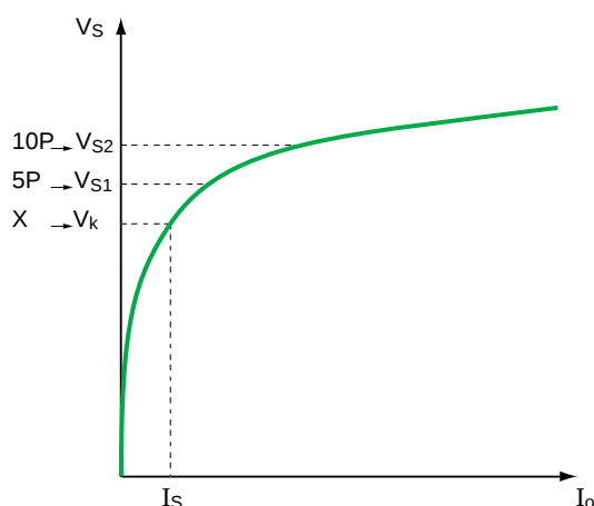
Fig. 7 : voltages corresponding to different CT classes.
