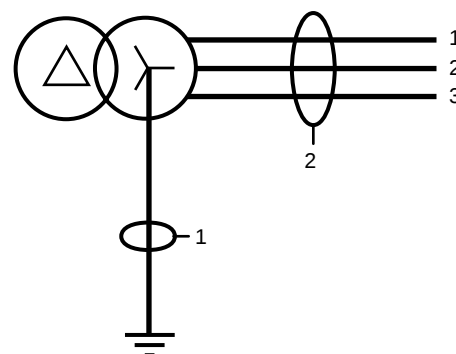
Fig. 16 : the toroid placed in (1) or (2) gives the same information... but the toroid placed in (1) also monitors the faults located upstream of the toroid (2).
