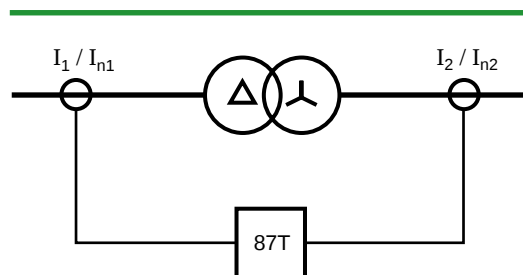
Fig. 29 : transformer differential protection principle.
